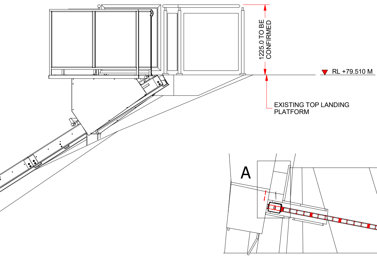
DETAIL-B TOP LANDING SCALE 1 : 40
