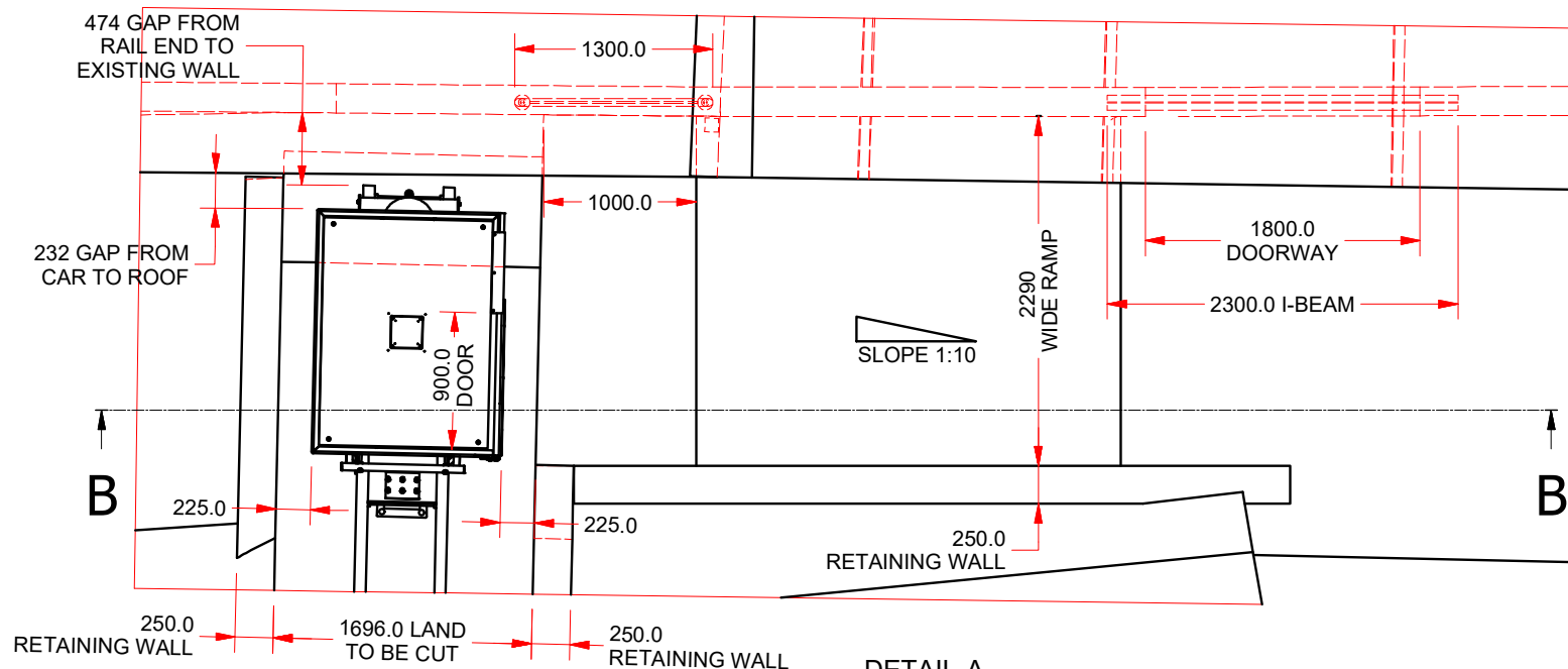
DETAIL-A BOTTOM LANDING SCALE 1 : 50
