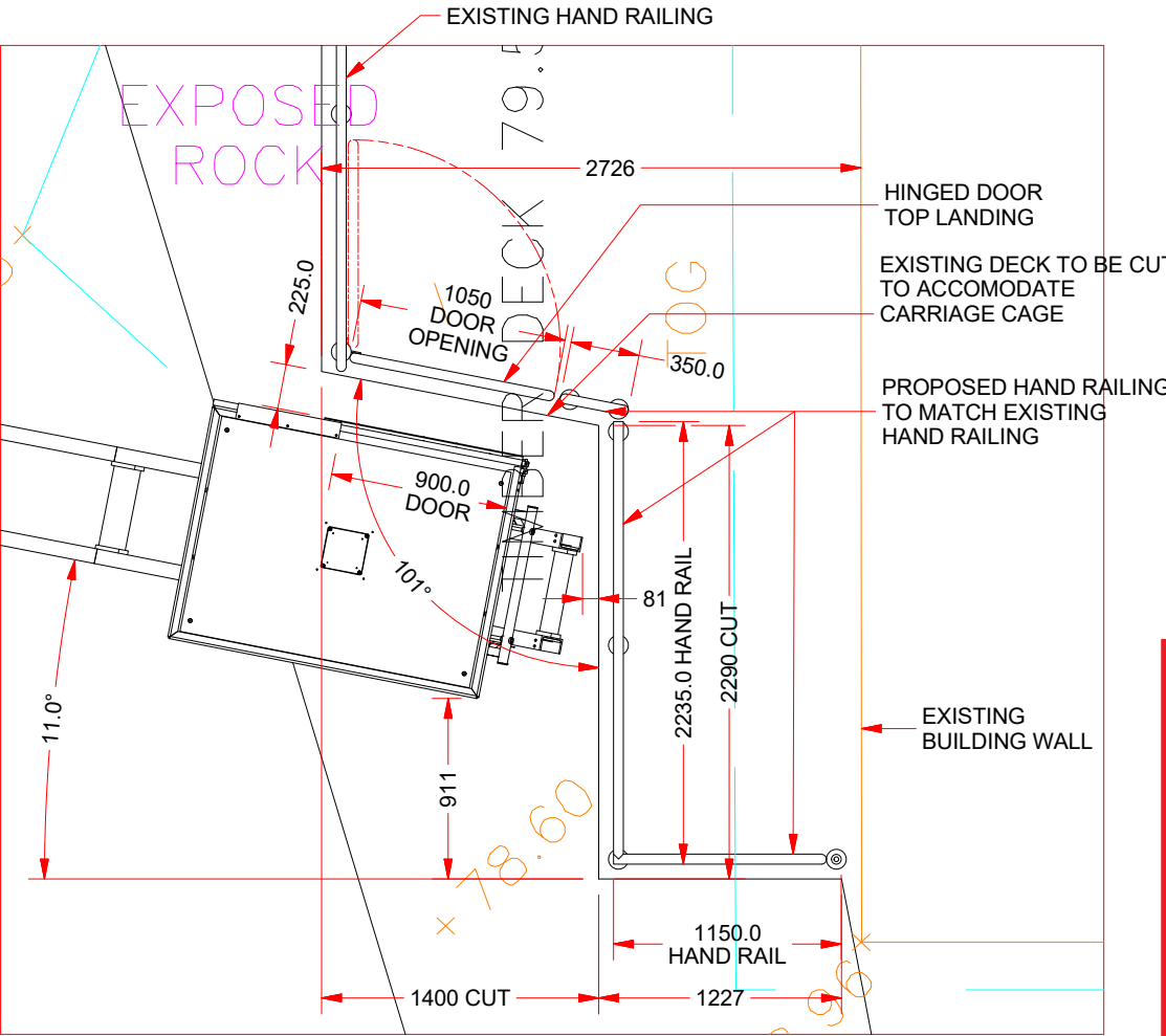
DETAIL-B TOP LANDING SCALE 1 : 40
