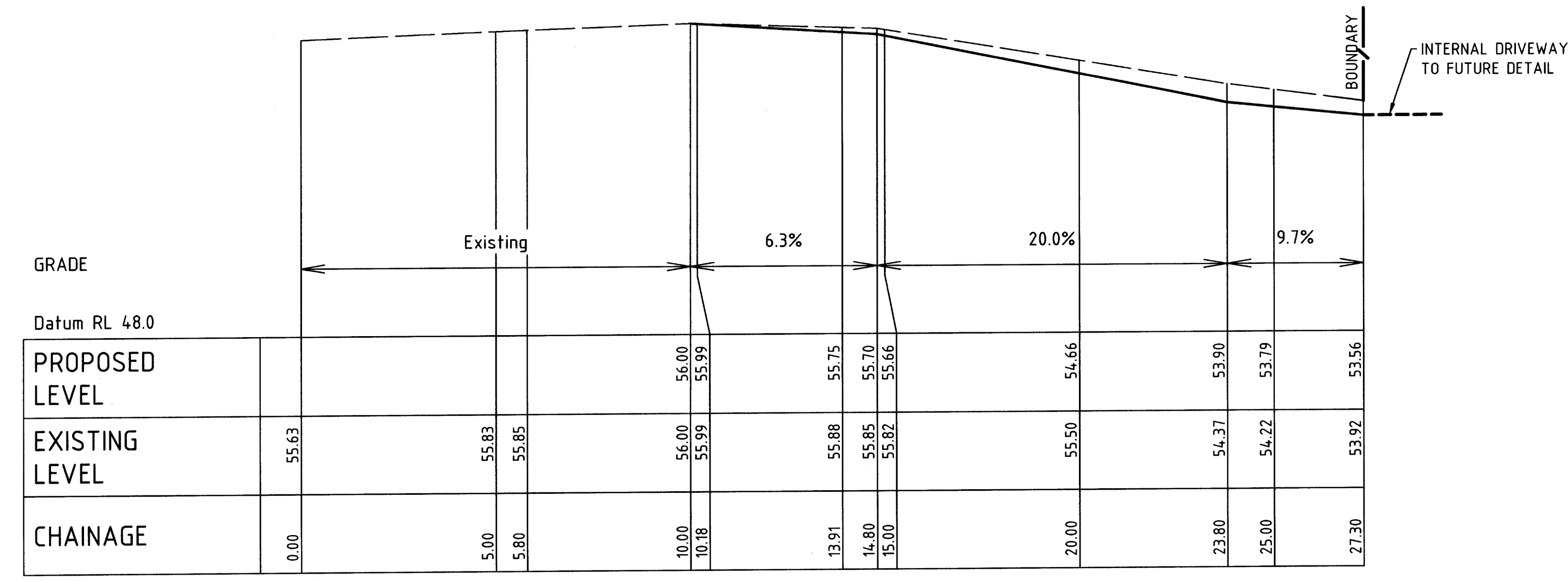
LONGITUDINAL SECTION ALONG DRIVEWAY
