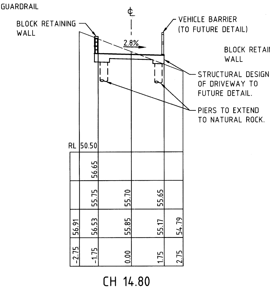
CROSS SECTIONS 1:100
