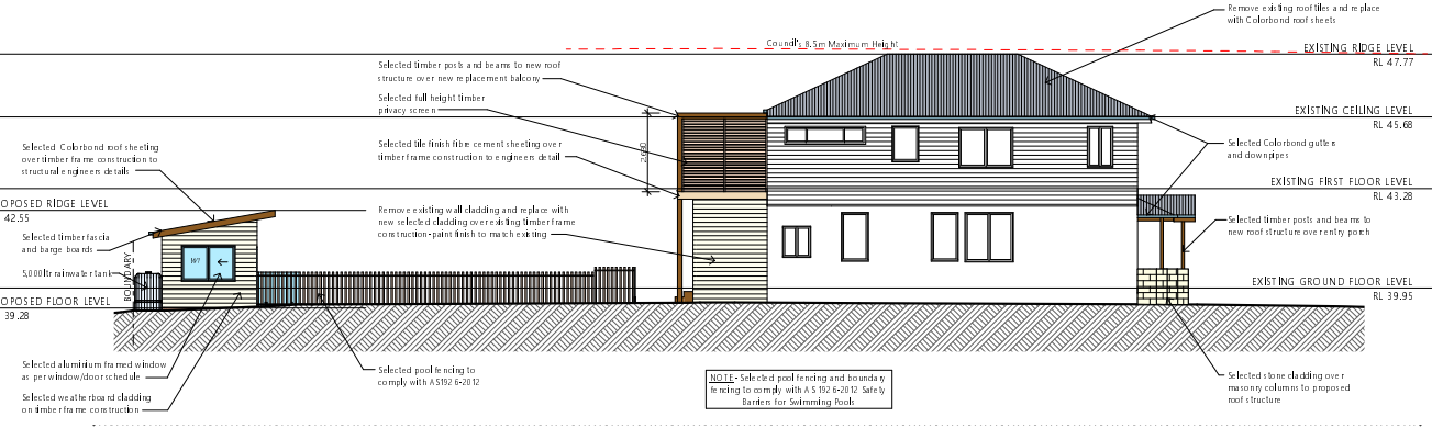
3 WEST ELEVATION 1:100
