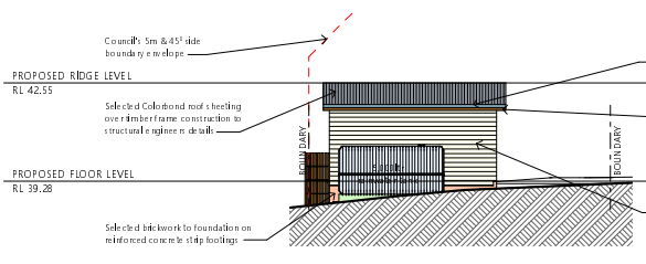
5 CABANA NORTH ELEVATION 1:100
