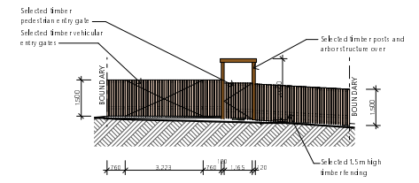
7 FRONT FENCE ELEVATION 1:100
