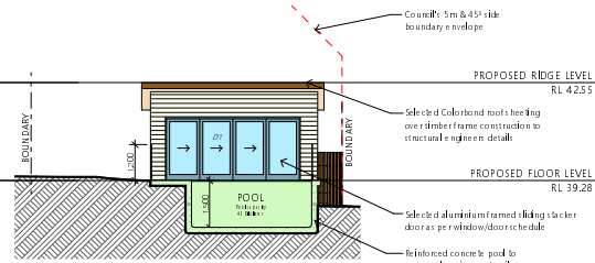
6 CABANA SOUTH ELEVATION 1:100
