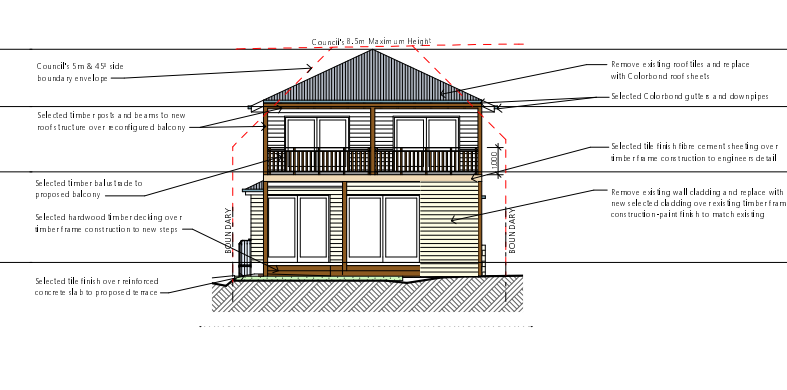
4 NORTH ELEVATION 1:100
