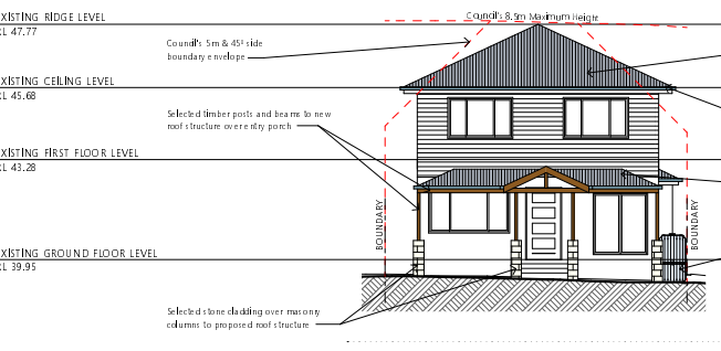
1 SOUTH ELEVATION 1:100
