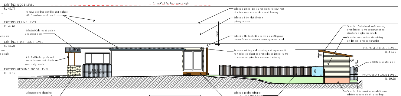
2 EAST ELEVATION 1:100
