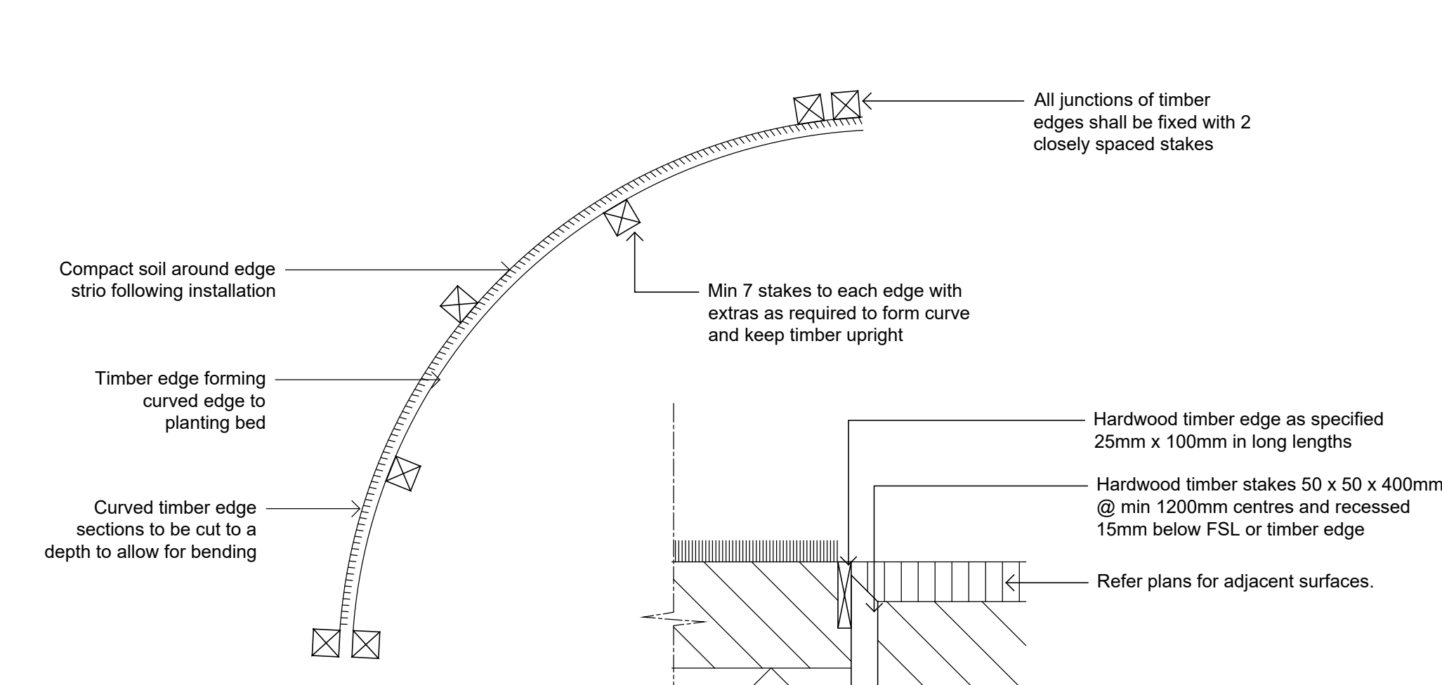
4 TIMBER EDGE - PLAN & SECTION SCALE 1:10
