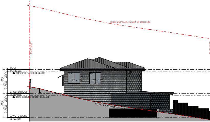
E EAST ELEVATION 1:250
