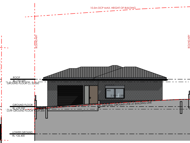
S SOUTHELEVATION 1:250
