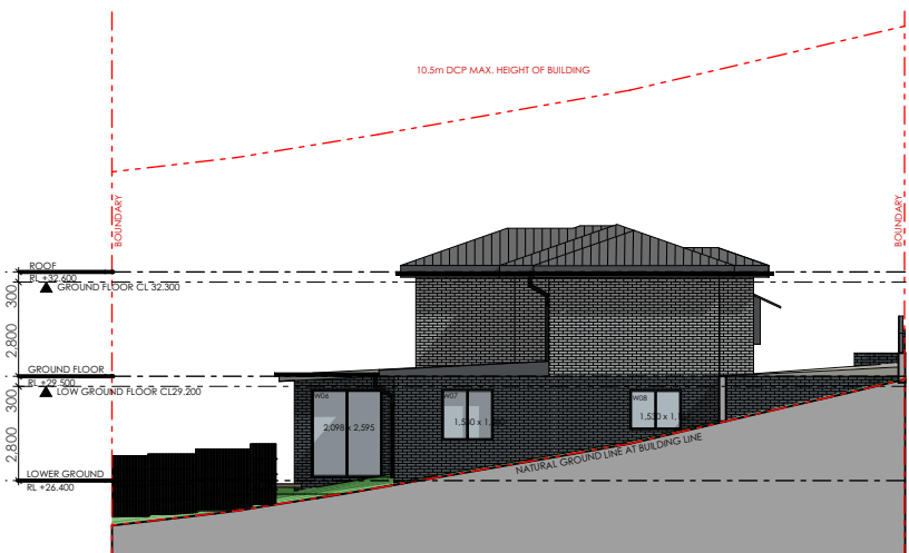
W WESTELEVATION 1:250
