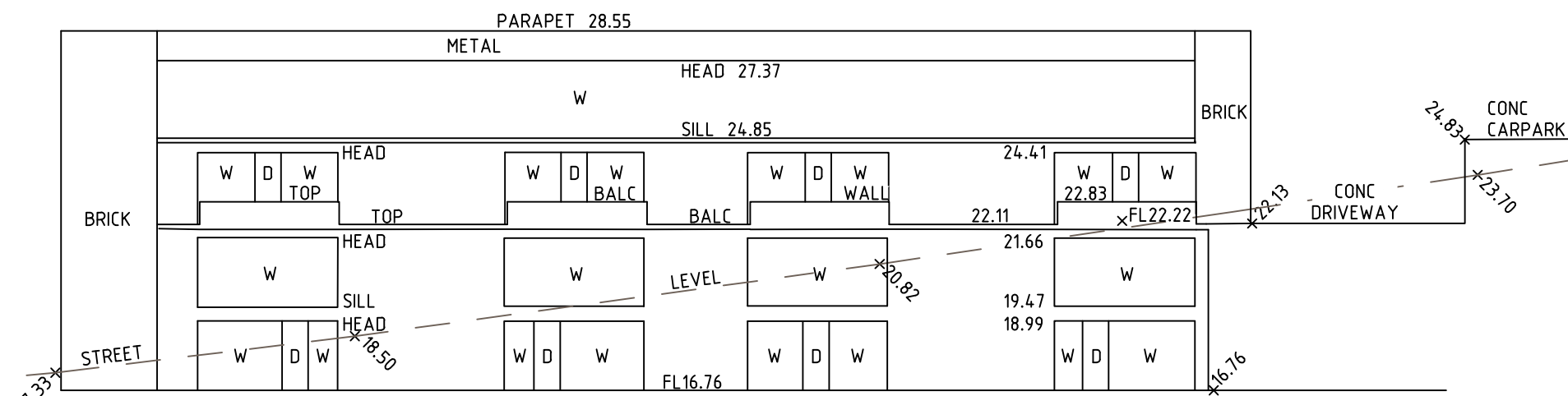
NORTHERN ELEVATION 3-9 KENNETH ROAD
