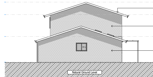
E-02 East 1:200
