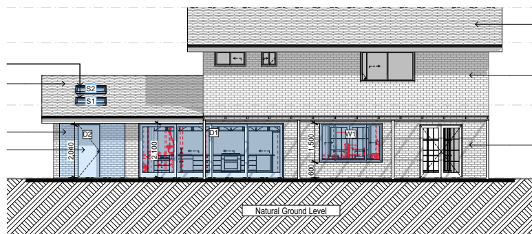
E-01 North 1:200
