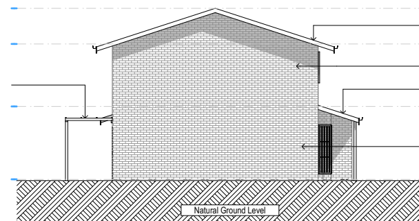
E-04 West 1:200
