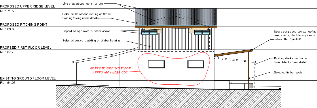
2 WEST ELEVATION 1:100
