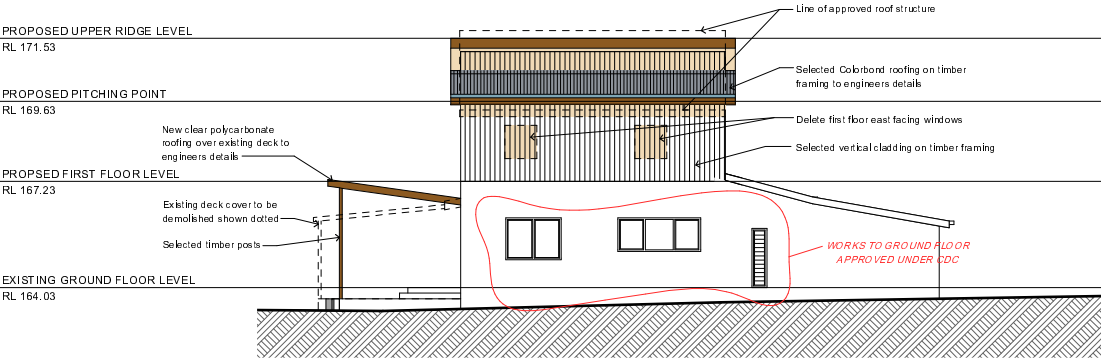
1 EAST ELEVATION 1:100
