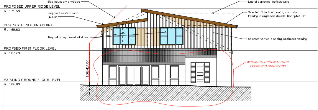
4 NORTH ELEVATION 1:100
