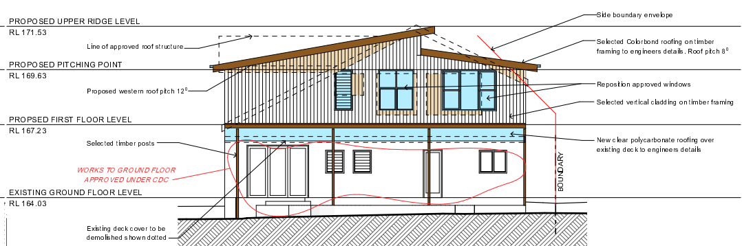
3 SOUTH ELEVATION 1:100
