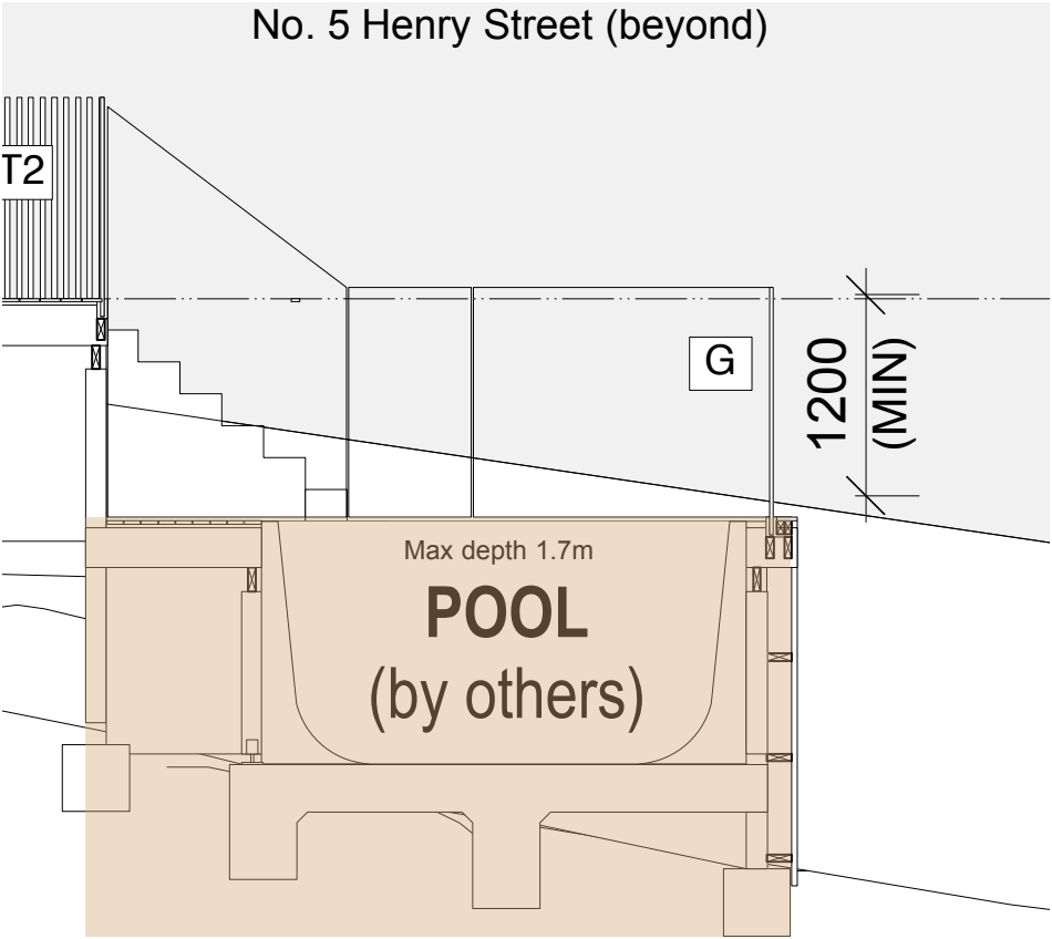
SECTION
