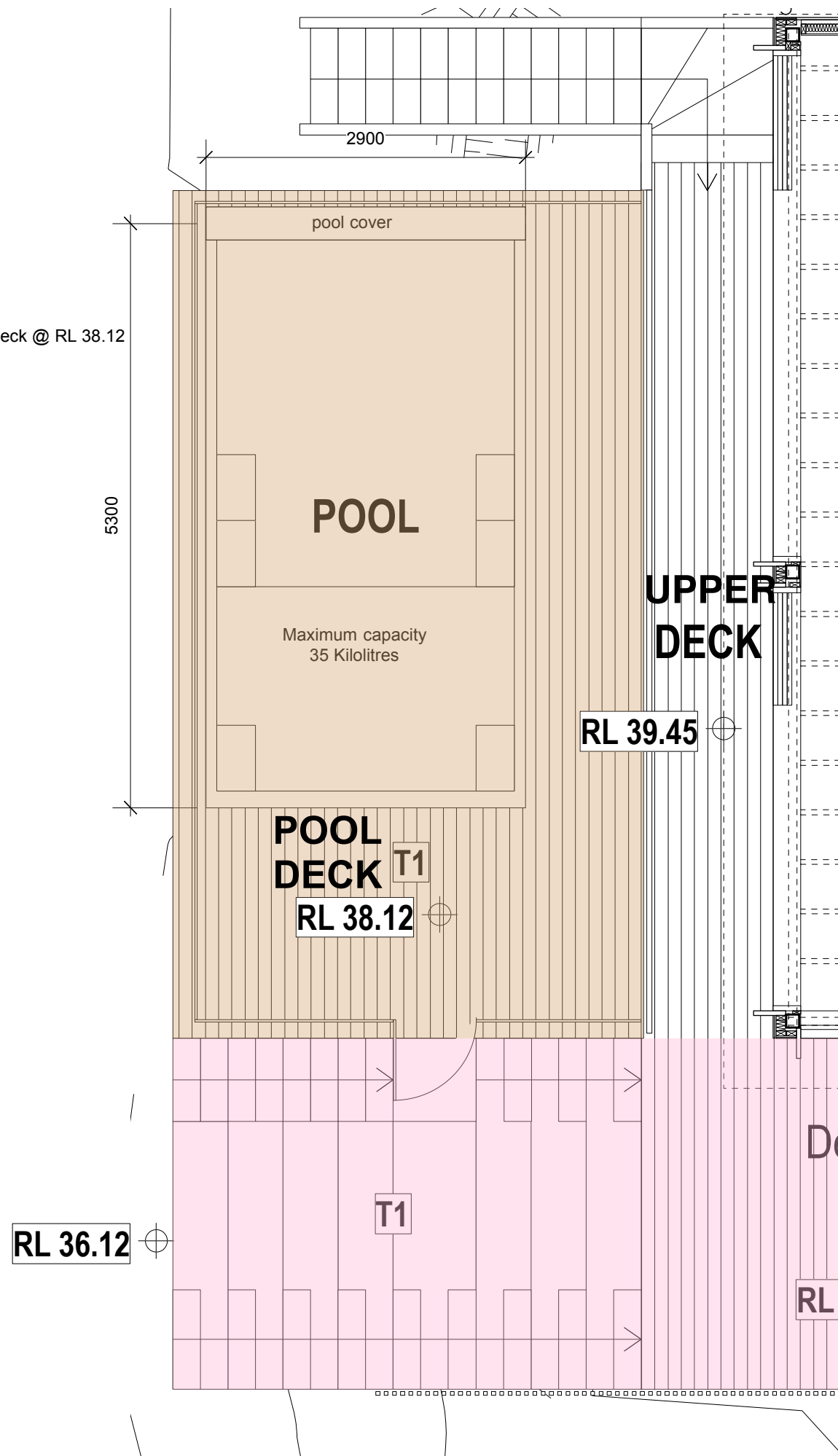
PLAN
