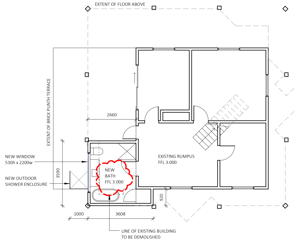
2 LEVEL 1 PROPOSED 1 : 100
