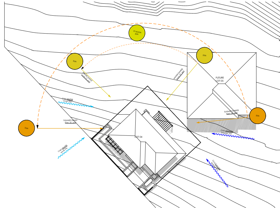
0 SITE ANALYSIS PLAN LOT 04, 10 FERN CREEK ROAD, WARRIEWOOD 1:500
