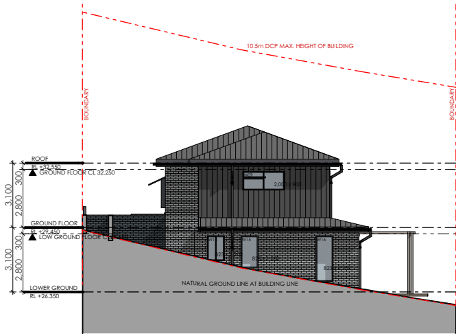
S SOUTH ELEVATION 1:250
