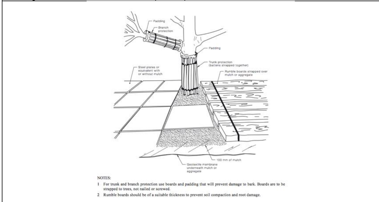
An image from AS4970-2009, 9 with example tree protection.
