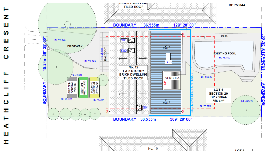
Figure 2: Site plan.
