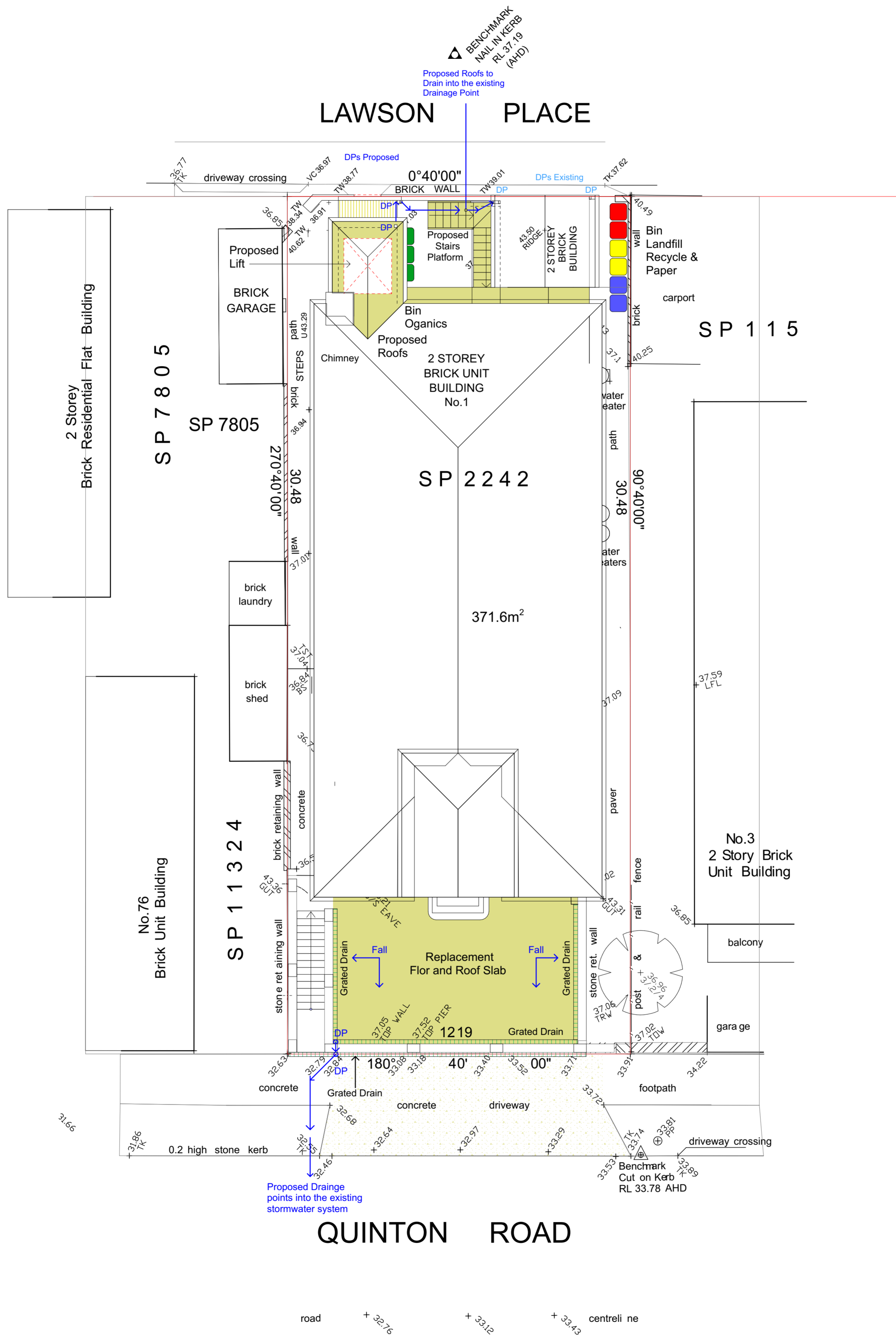
Stormwater Plan
