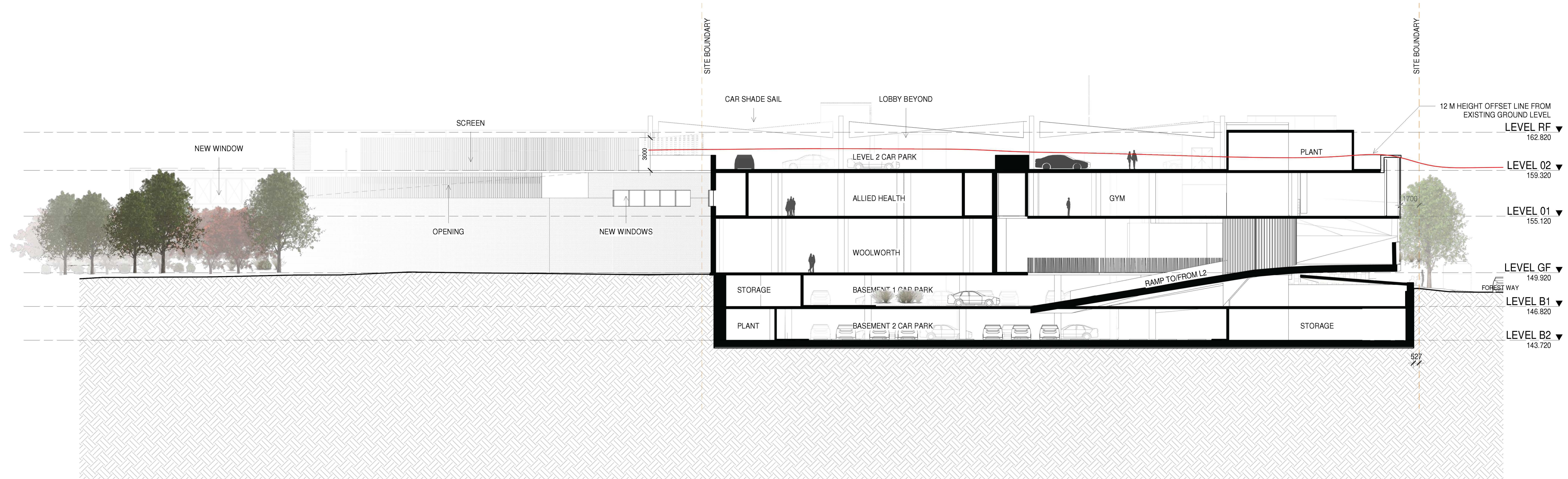
F-F SECTION F SCALE 1:200
