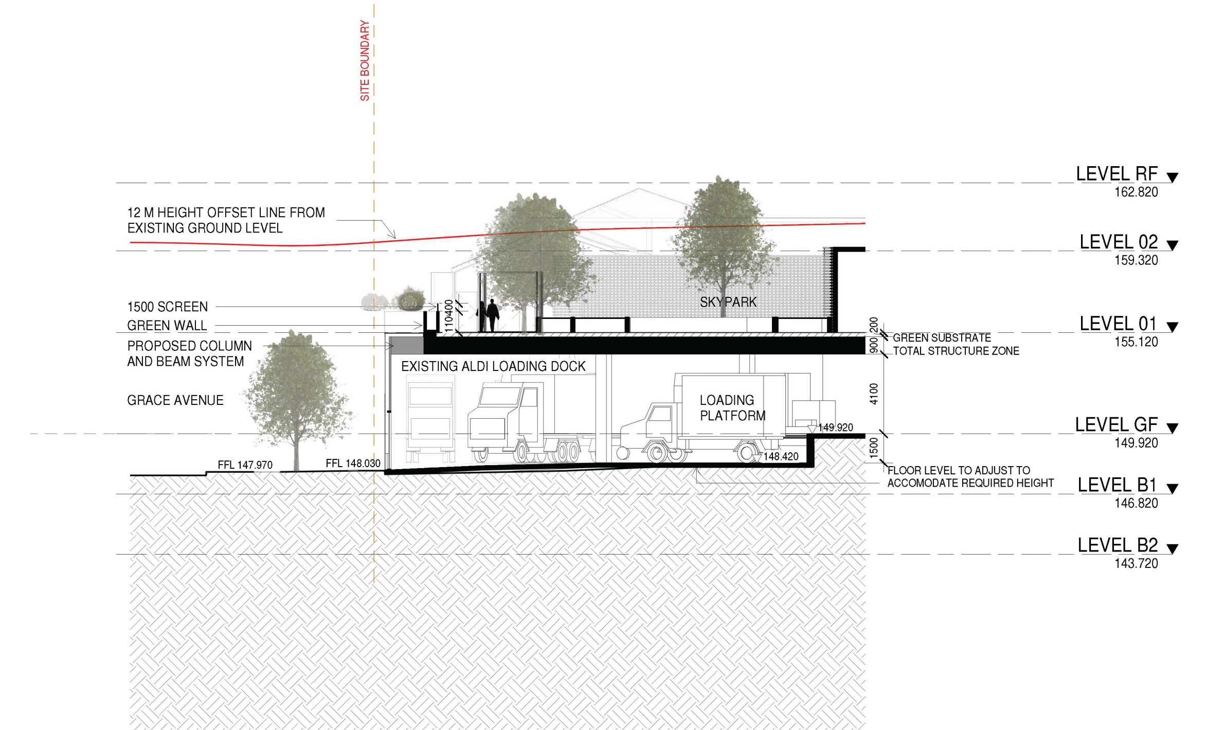
(D-D) SECTION D ASK-20007 SCALE 1:200
