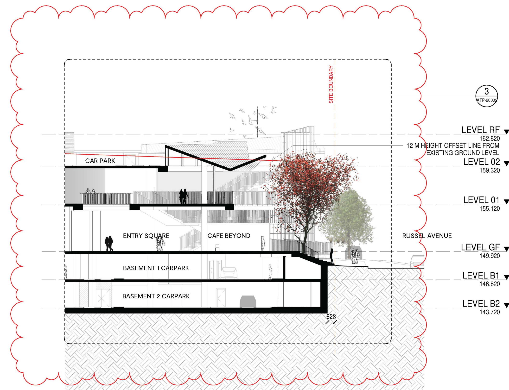
(B-B) SECTION B ASK-20007 SCALE 1:200
