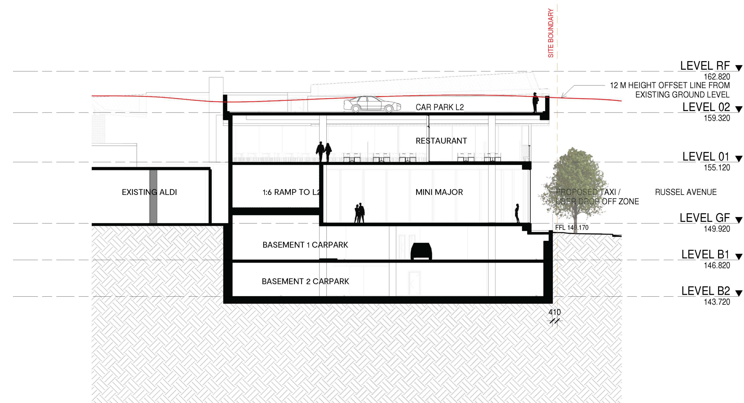
(C-C) SECTION C ASK-20007 SCALE 1:200
