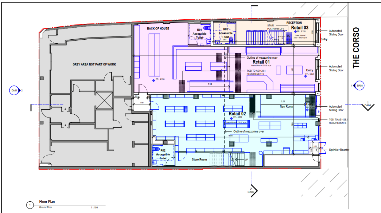
Figure 1 Proposed Floor Plan (Antoniadis Architects, 27/05/2024)
