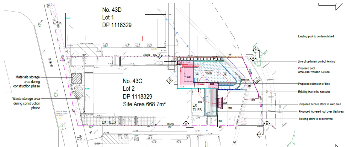
Figure 3: Site plan
