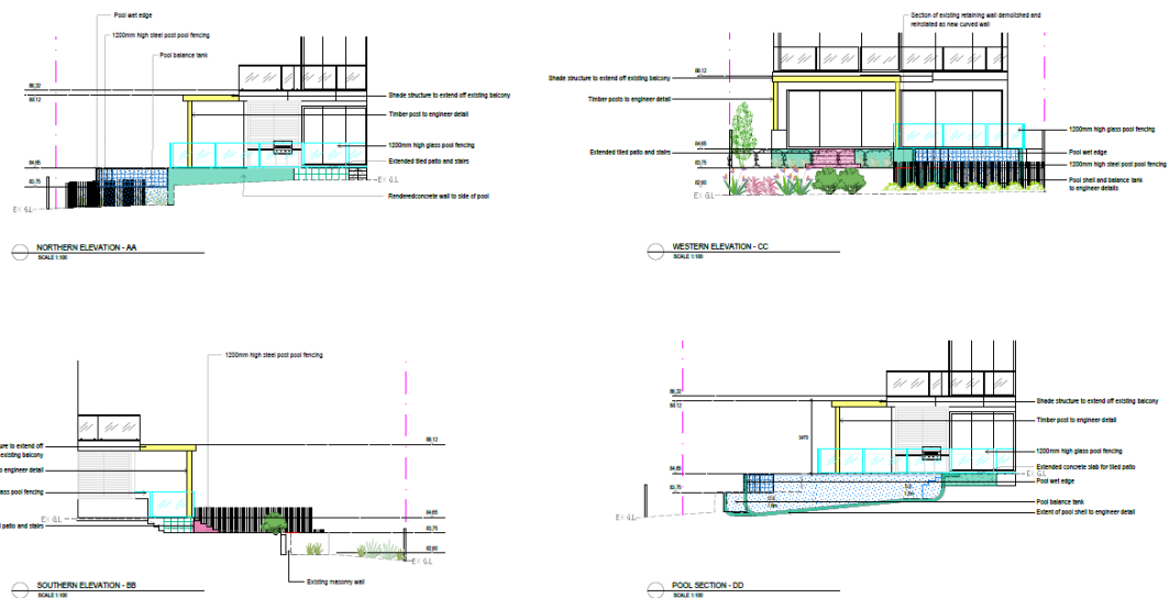
Figure 4: Elevations
