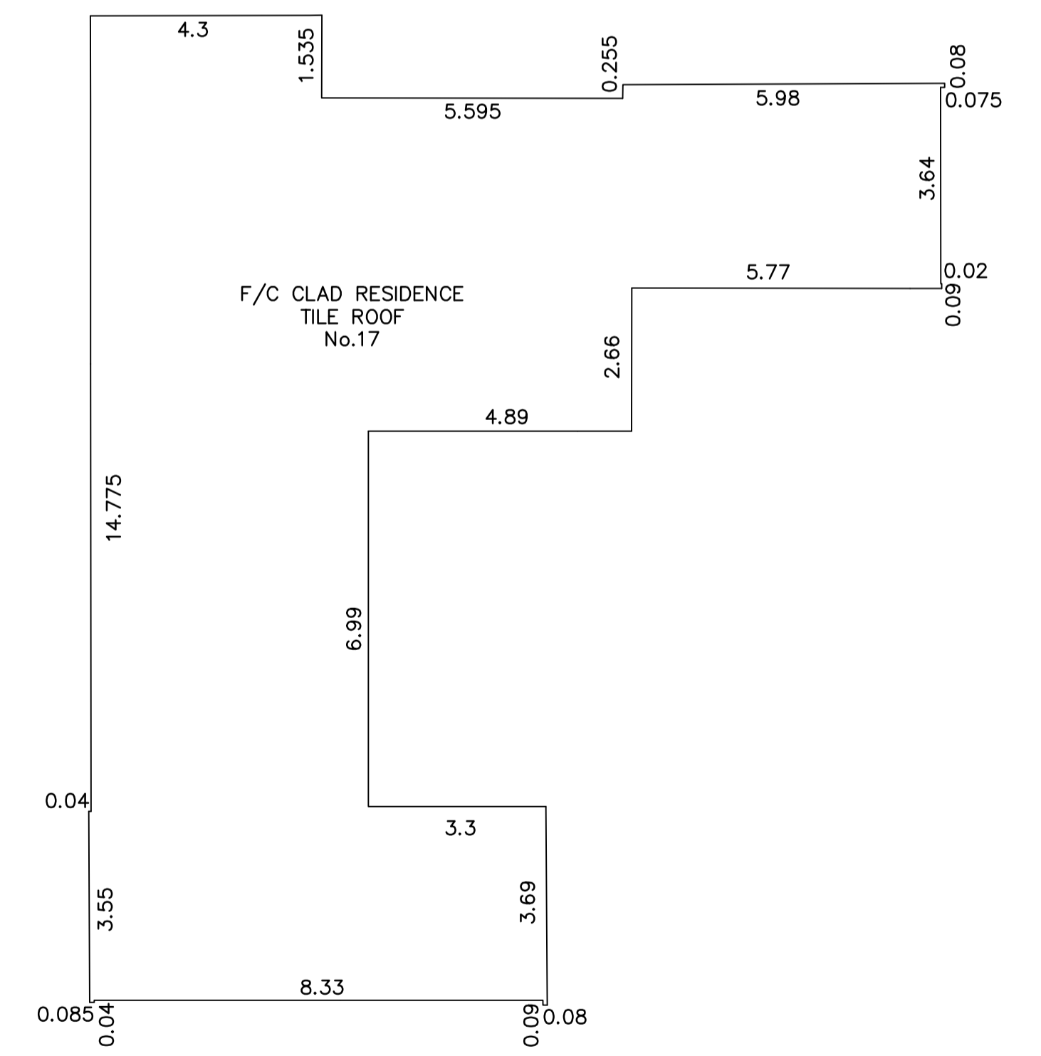
SKETCH SHOWING HOUSE DIMENSIONS
