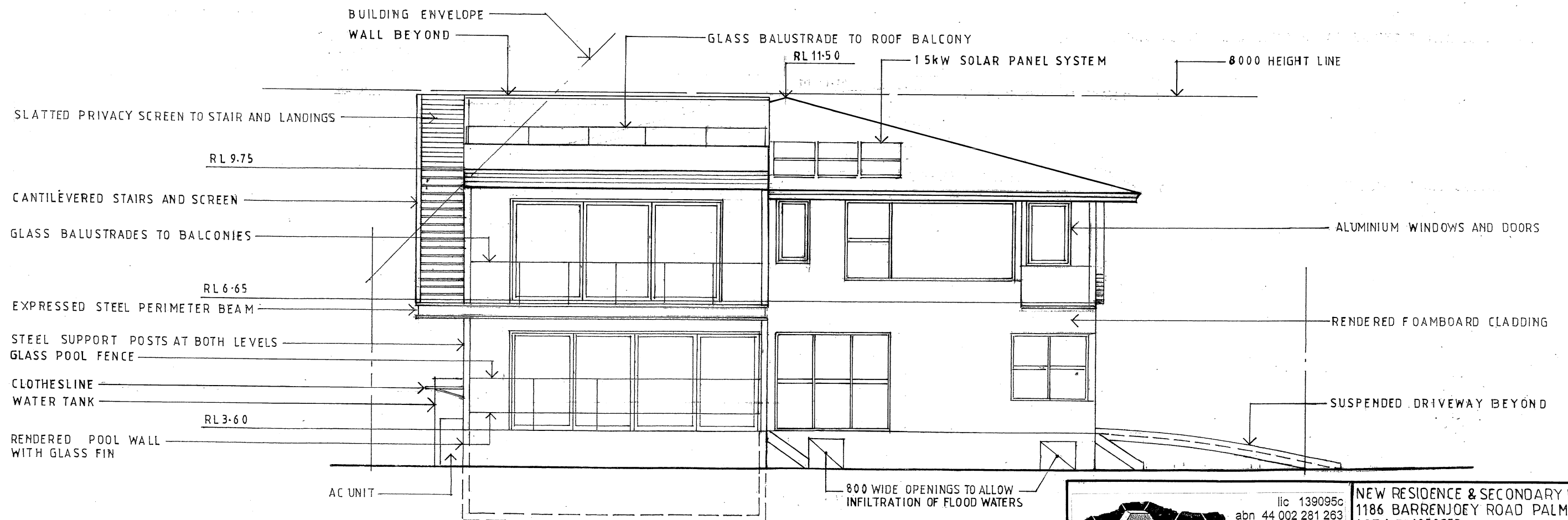
NORTH ELEVATION
