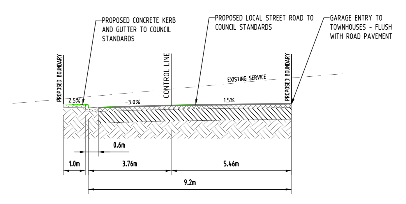
TYPICAL SECTION - ROAD 2 @ CH70
