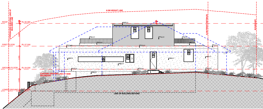
NORTH ELEVATION
