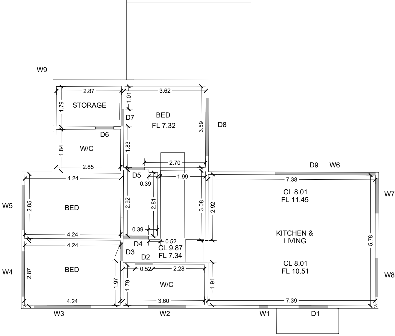
FIRST FLOOR
