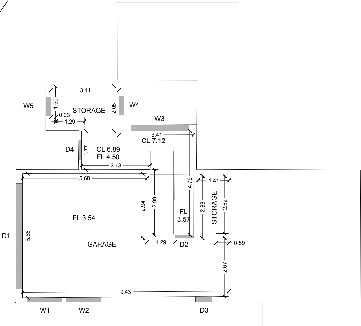
GROUND FLOOR & GARAGE
