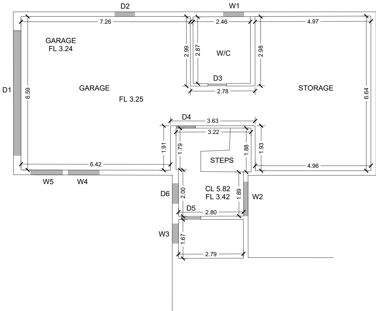
GROUND FLOOR & GARAGE
