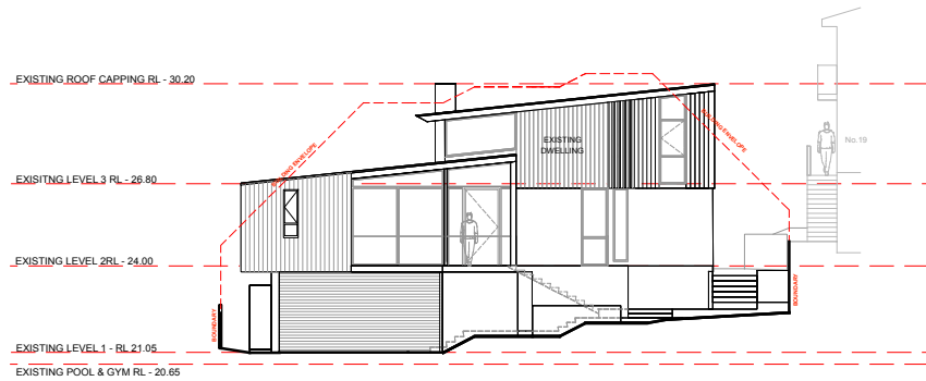
WEST ELEVATION
