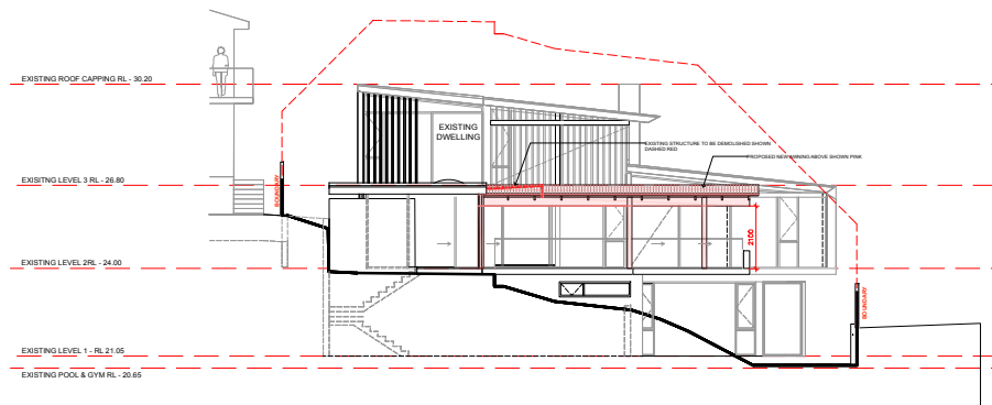
EAST ELEVATION
