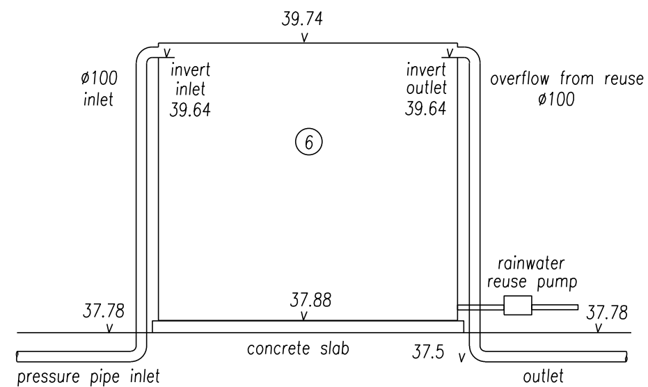
section through rainwater reuse tank not to scale
