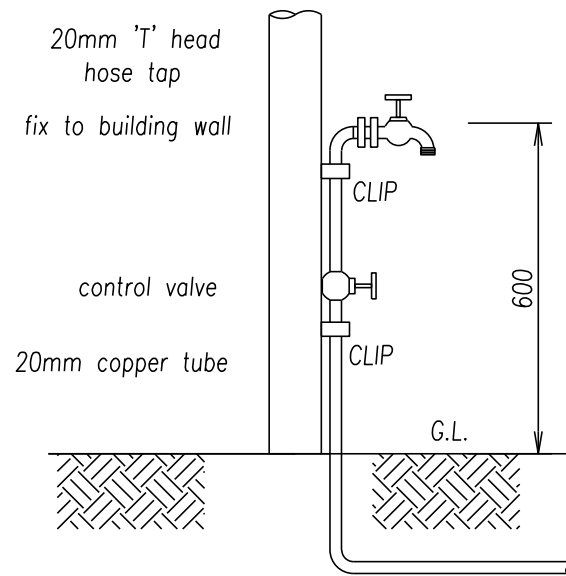
hose tap detail not to scale
