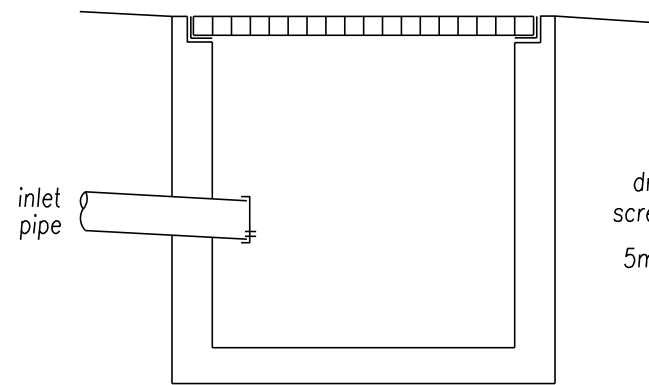
dribble pipe details not to scale
