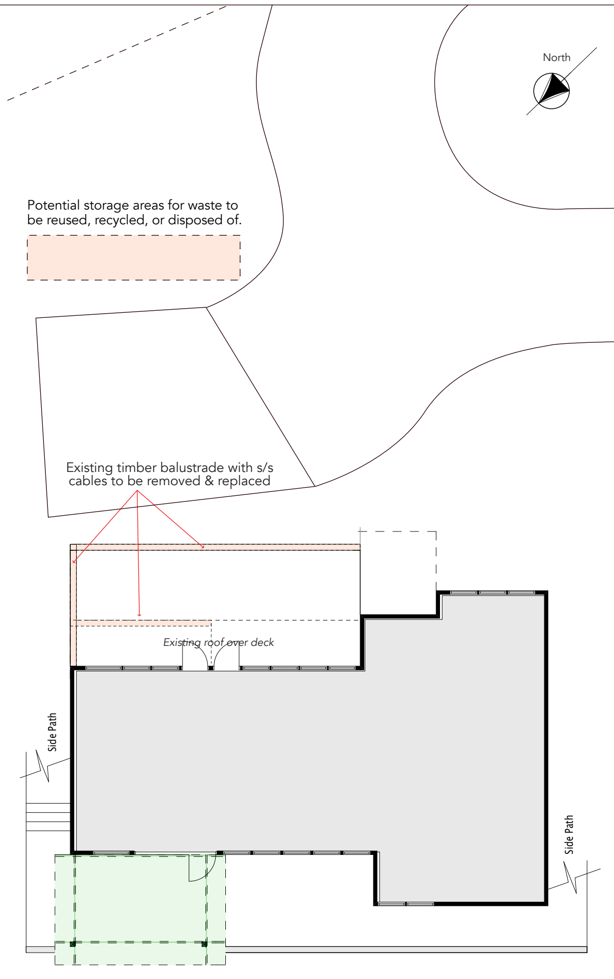
Site Plan indicating existing balustrade to be demolished & potential waste & materials storage
