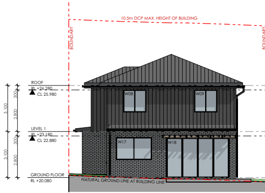
2 EAST ELEVATION 1:250
