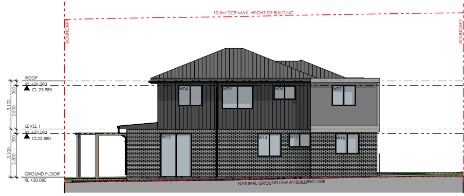
3 NORTH ELEVATION 1:250
