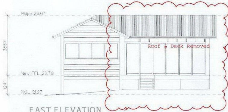
EAST ELEVATION
