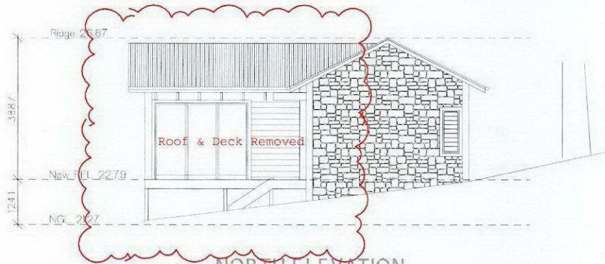
NORTH ELEVATION
