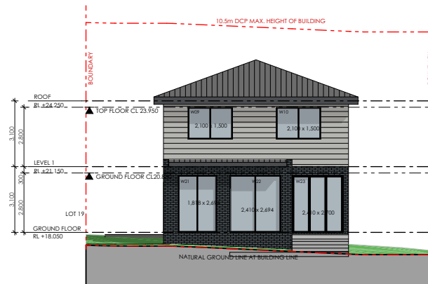
2 EAST ELEVATION 1:250
