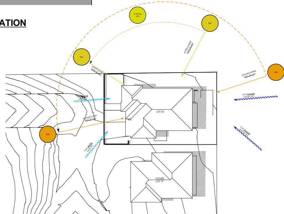
5 SITE ANALYSIS PLAN 1:500
