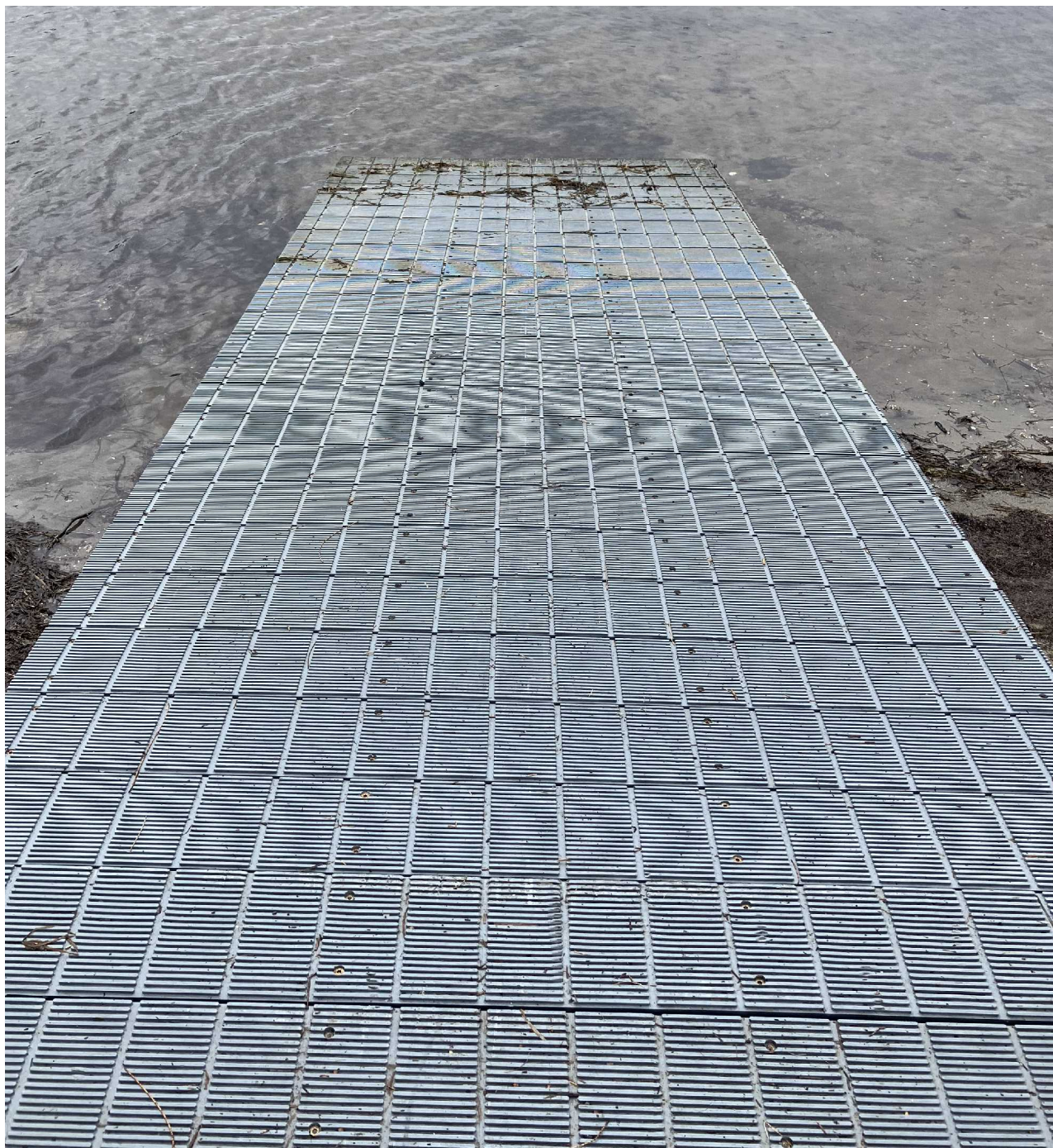
DESIGN INTENT FOR WATER ACCESS PLATFORM
