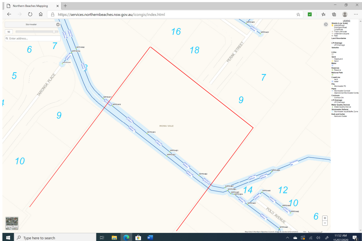
Figure 2: Enlarged Northern Beaches Council Stormwater Map, Stormwater Infrastructure (Blue) and Depot Boundary (in Red).
