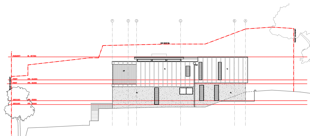
WEST ELEVATION
