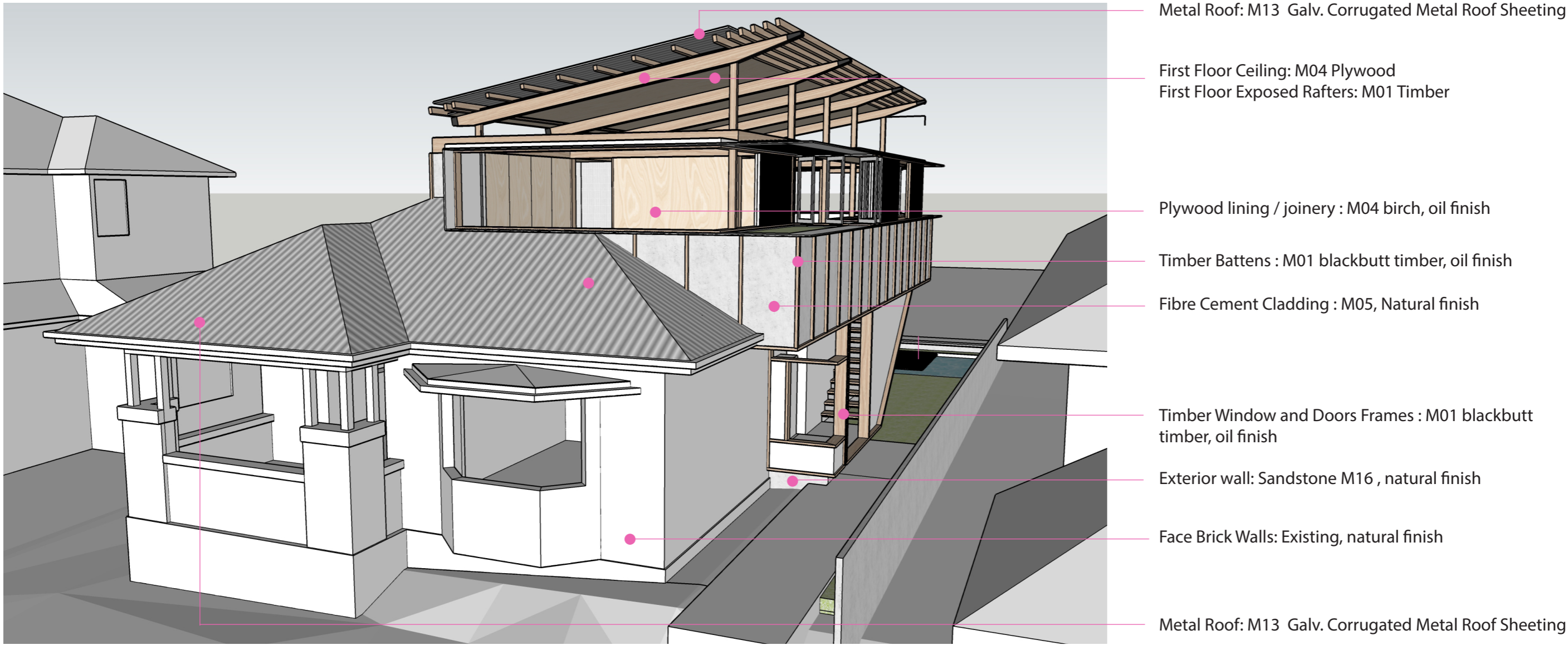
Materials Diagram
