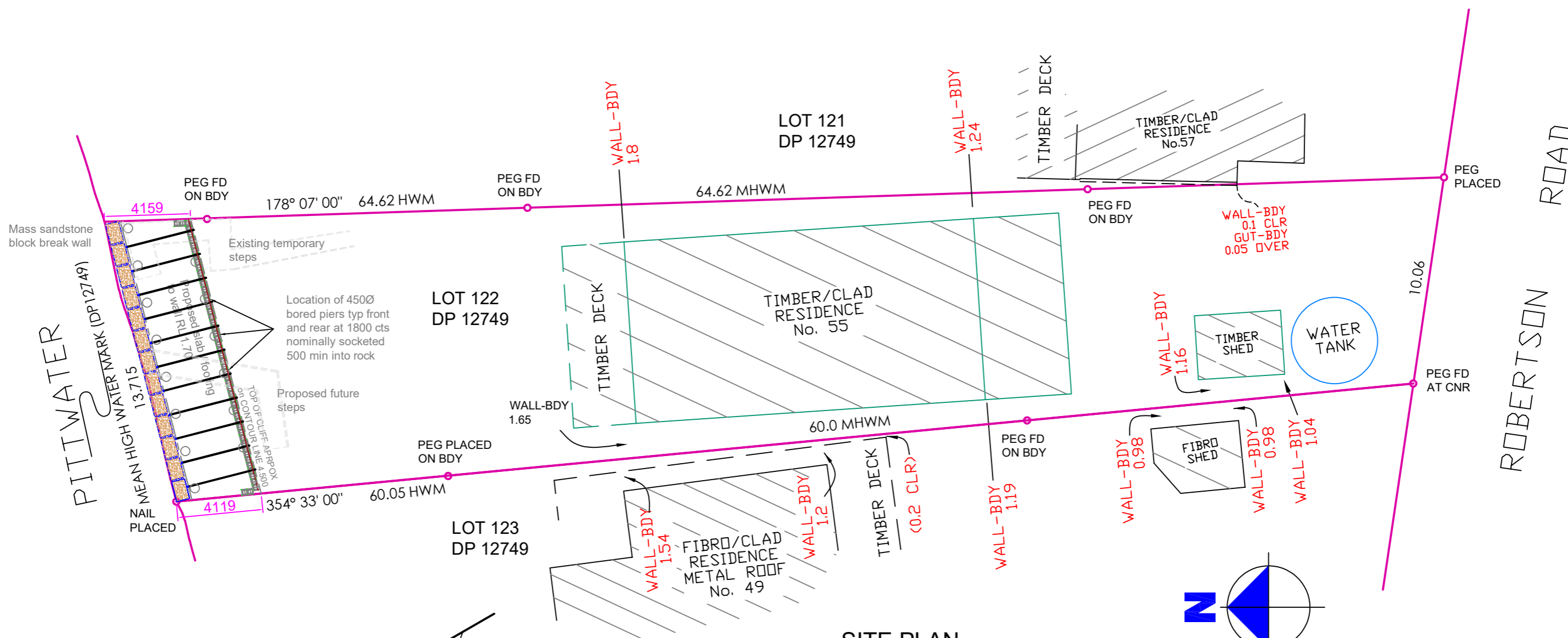
SITE PLAN Scale: 1 in 200
