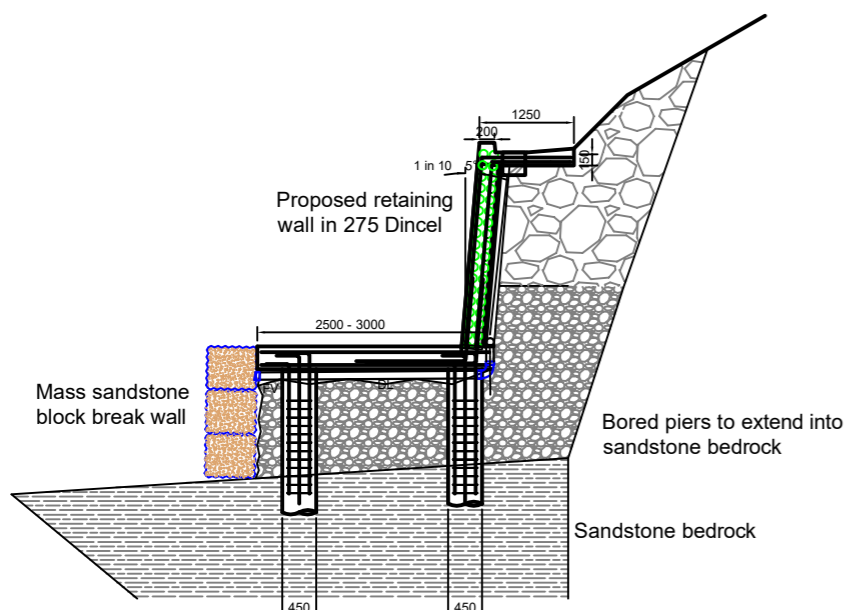
SECTION THROUGH WALL Scale: 1 in 100
