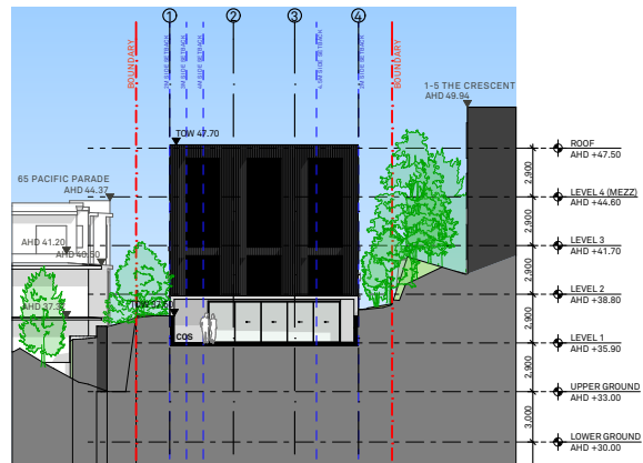
SOUTH ELEVATION
