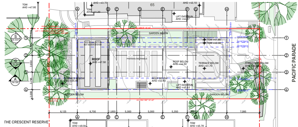
SITE PLAN
