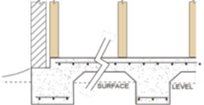
Fig. 1 Stiffened Raft
