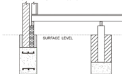
Fig. 3 Strip & Stump Footing System
