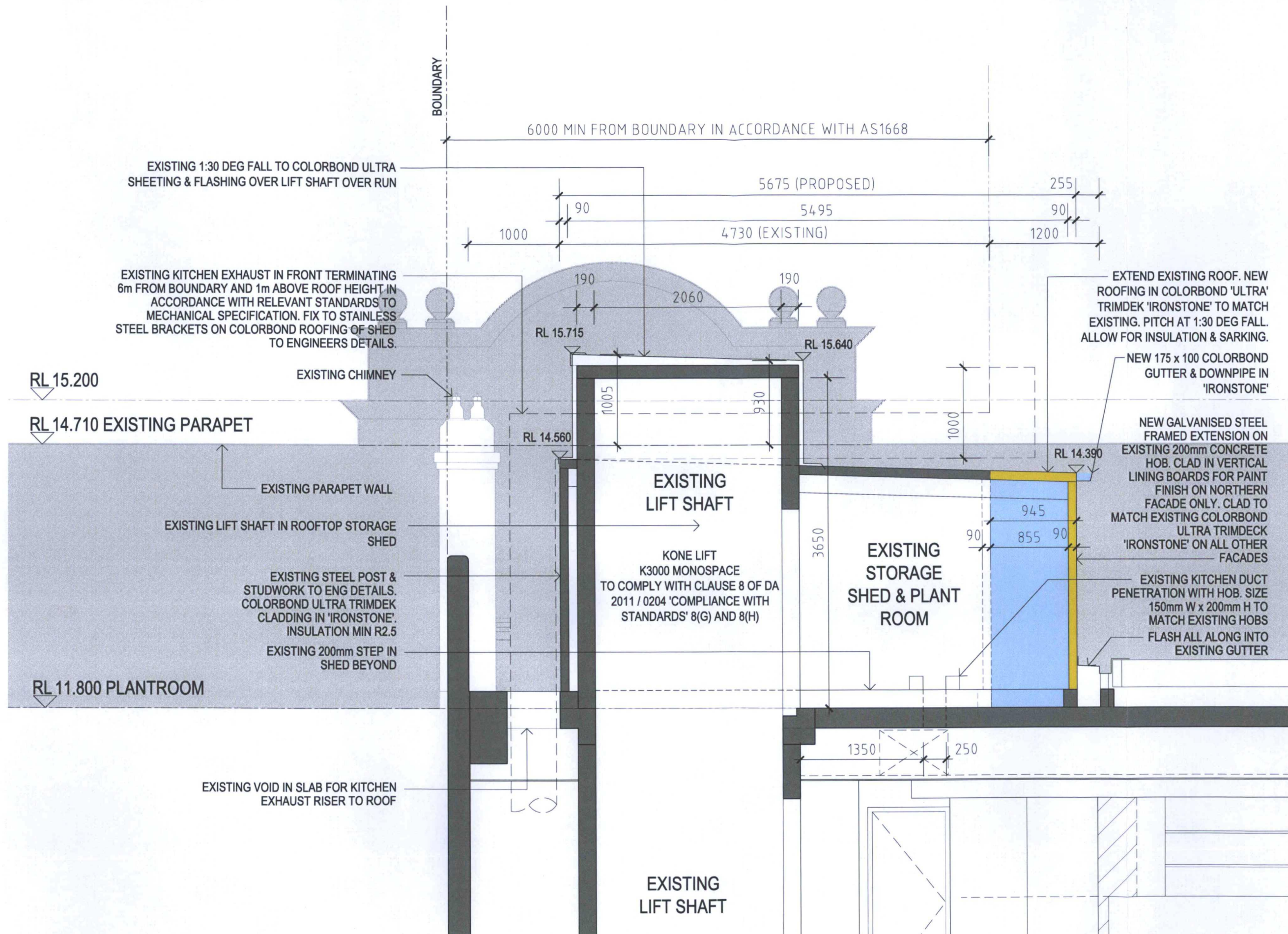
01 SHED & LIFT SECTION scale - 1:50 @ A3
