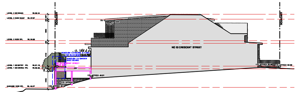
South Elevation
