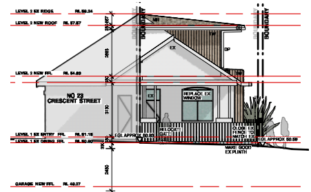
East Elevation - Crescent Street
