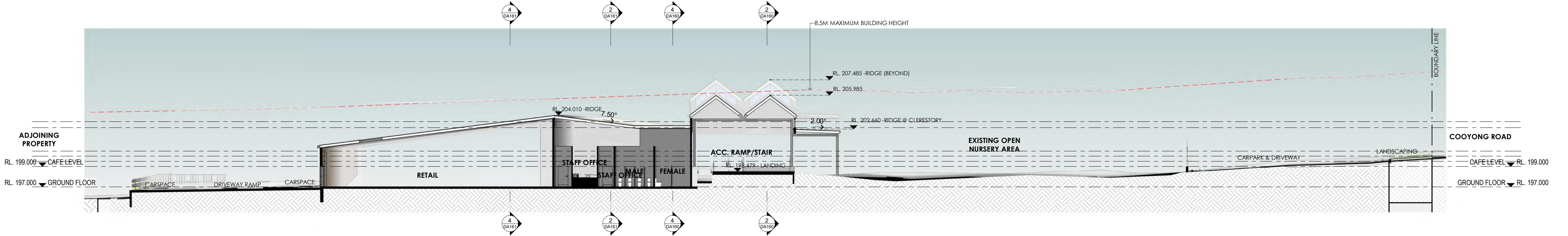
2 BUILDING SECTION 6 Scale: 1 : 200
