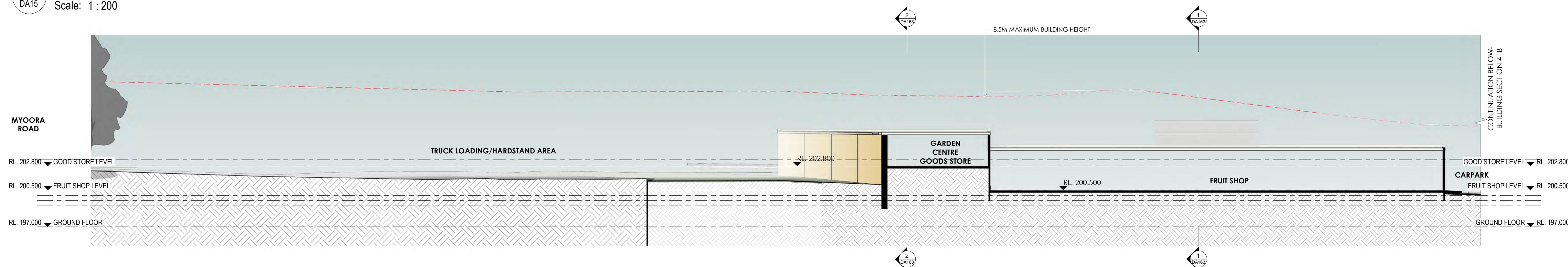
3 BUILDING SECTION 4-A Scale: 1 : 200
