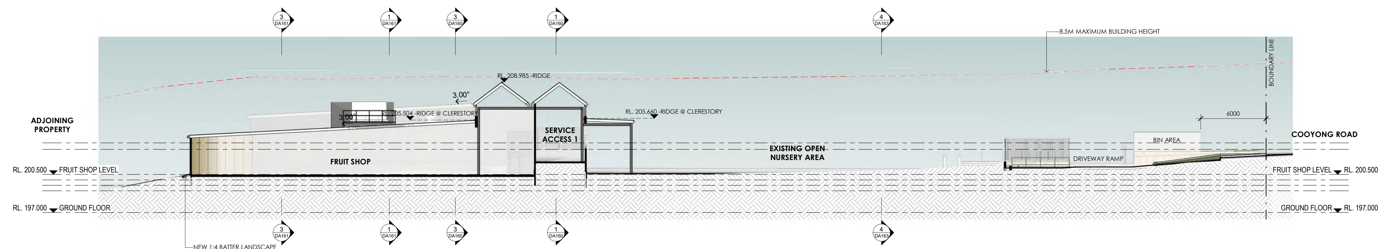
1 DA15 BUILDING SECTION 9 Scale: 1 : 200
