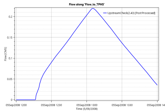
Figure 6 - Catchment A, 1% AEP contributing flows to B
