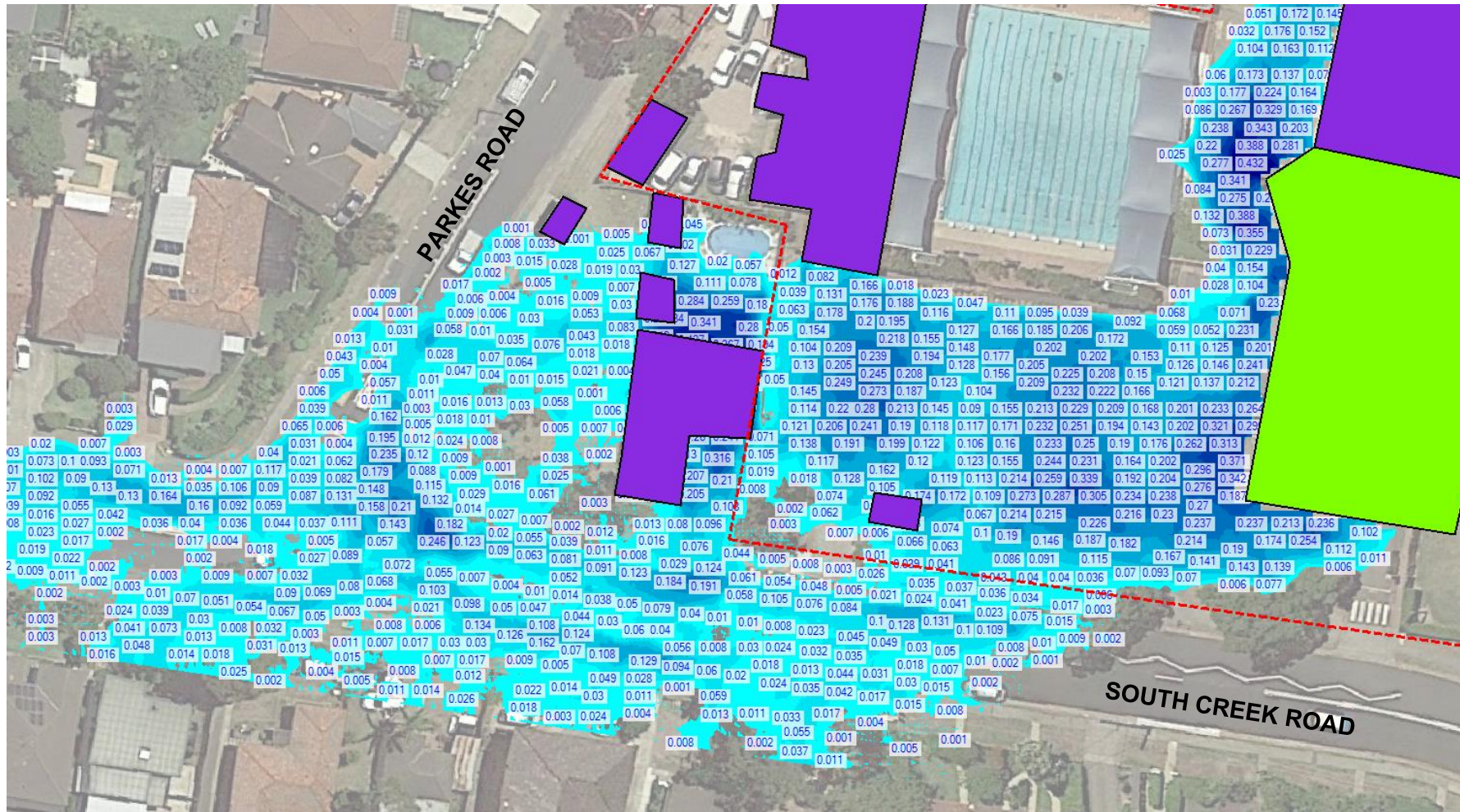
Figure 11 - Post-development, 1% AEP (blocked), depth (m) at South Creek Road
