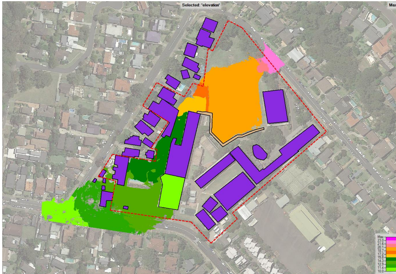
Figure 30 - Post-development, PMF, Water Surface Elevation (mAHD)
