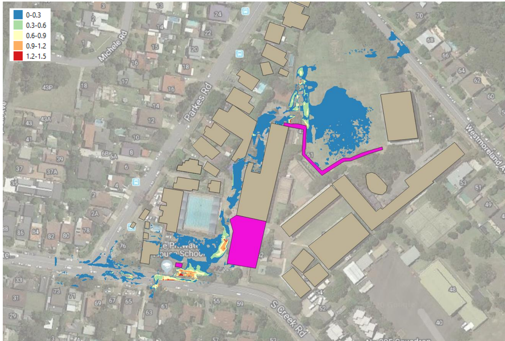
Figure 33 - Afflux Map (Post minus Pre), 1% AEP, Velocity (m/s)
