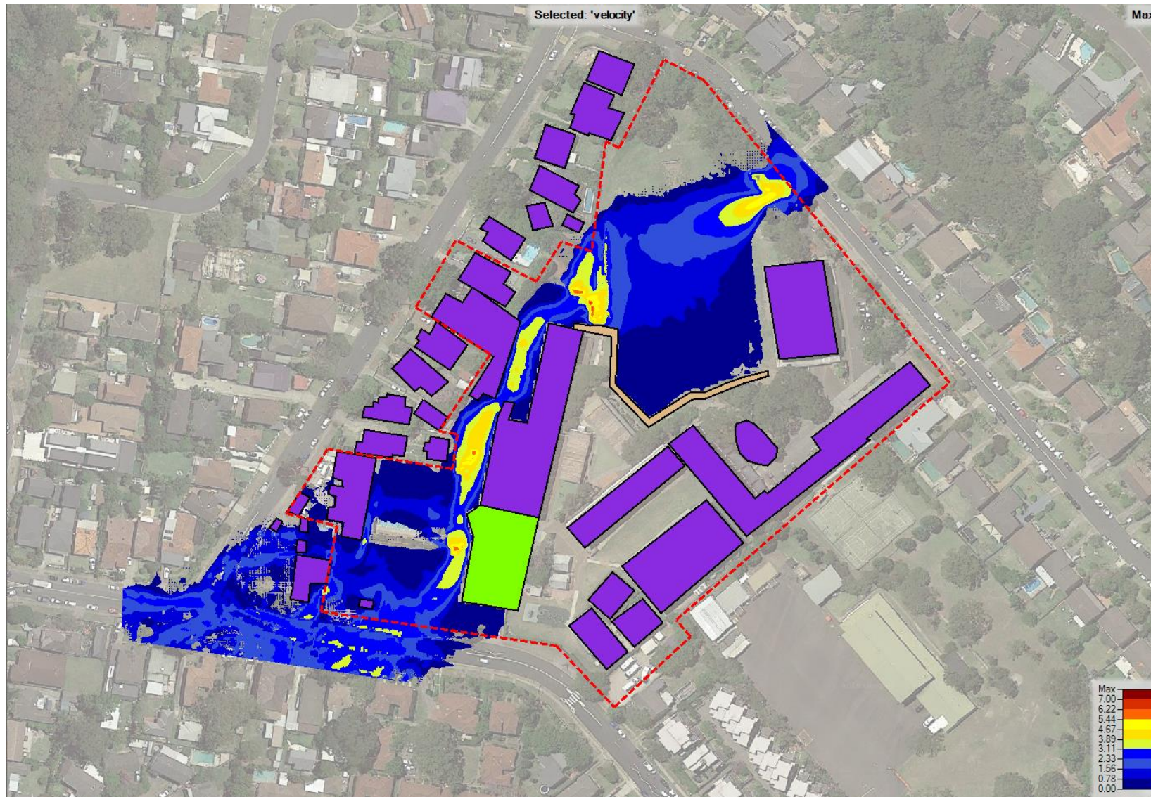
Figure 29 - Post-development, PMF, Velocity (m/s)
