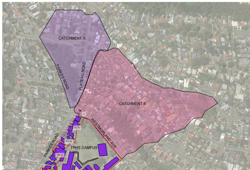
Figure 4 - Catchment plan
