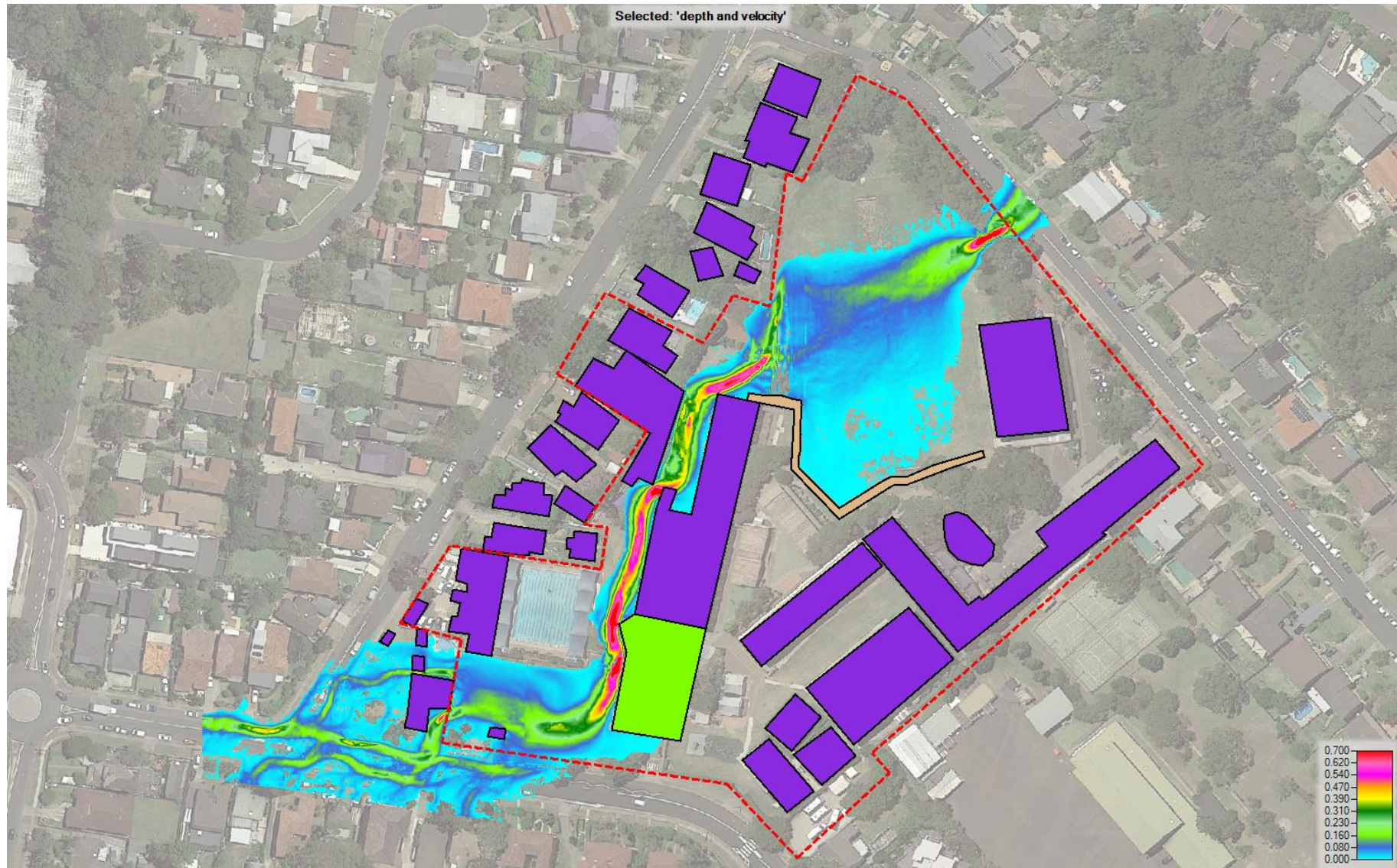
Figure 25 - Post-development, 1%AEP (blocked), Velocity Depth Product ( \text{m}^2/\text{s} )
