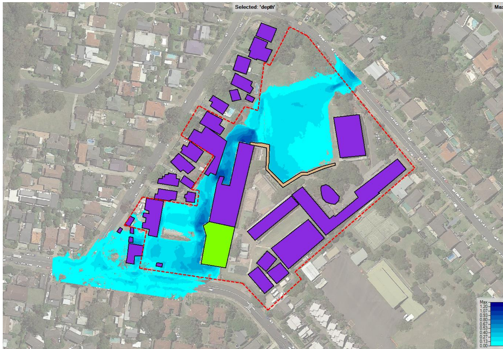
Figure 28 - Post-development, PMF, Depth (m)
