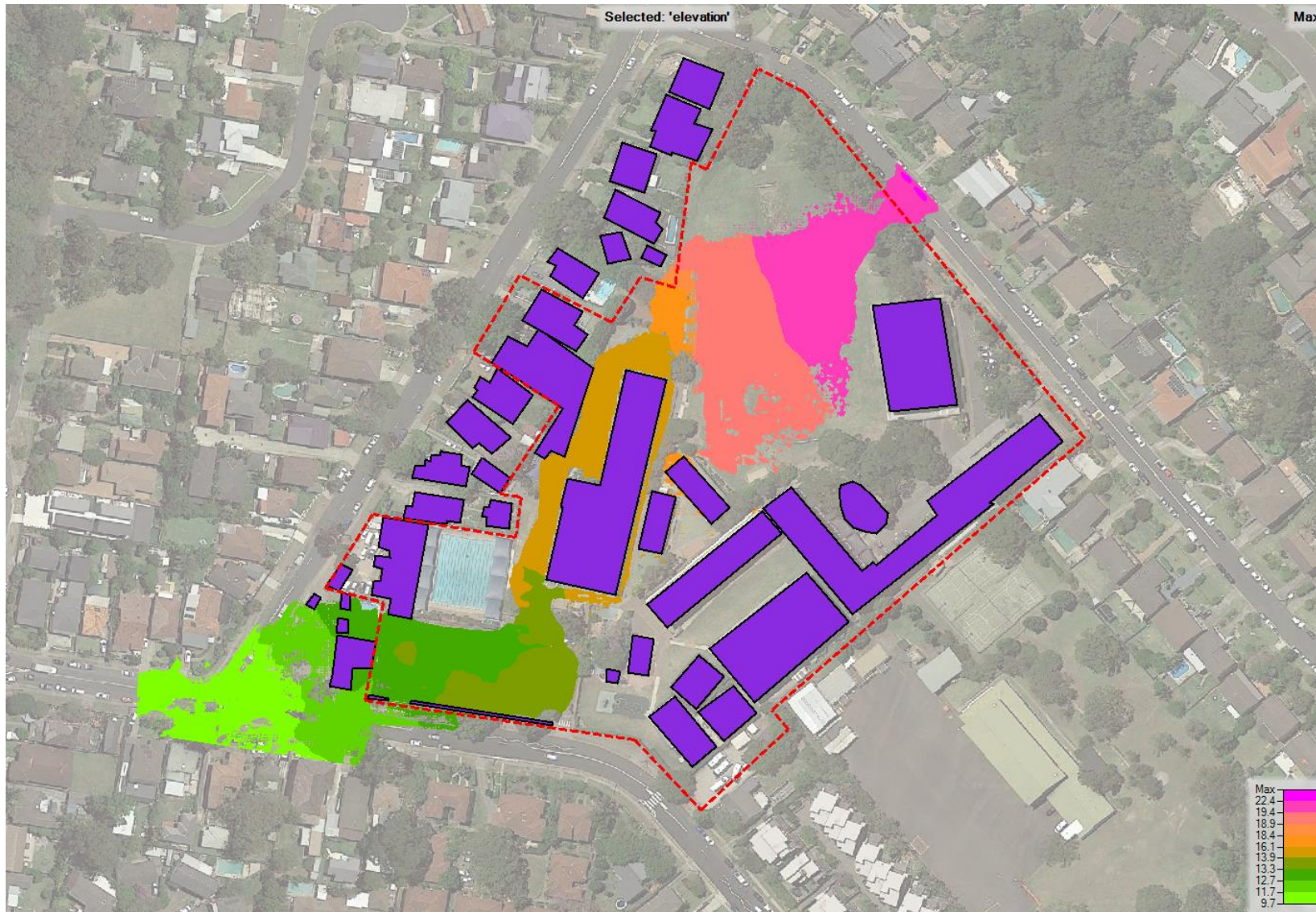
Figure 17 - Pre-development, 1%AEP (blocked), Water Surface Elevation (mAH)
