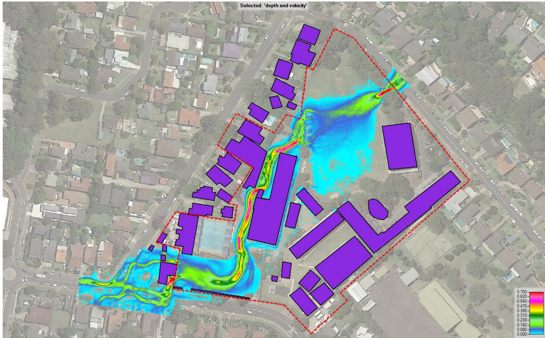
Figure 18 - Pre-development, 1%AEP (blocked), Velocity Depth Product ( \text{m}^2/\text{s} )
