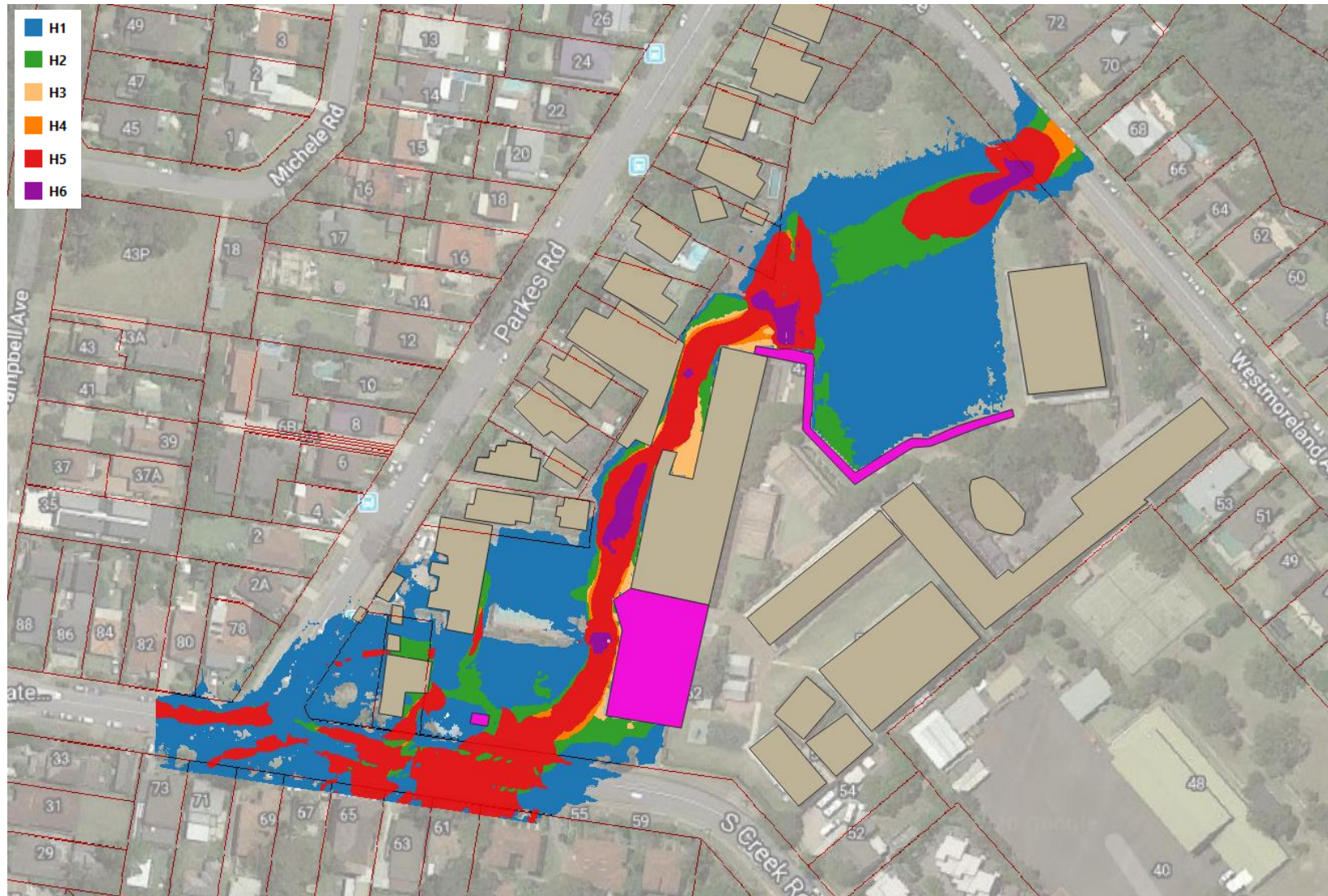
Figure 31 - Post-development, PMF, Flood Hazard
