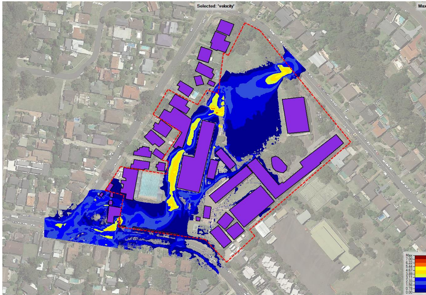
Figure 21 - Pre-development, PMF, Velocity (m/s)
