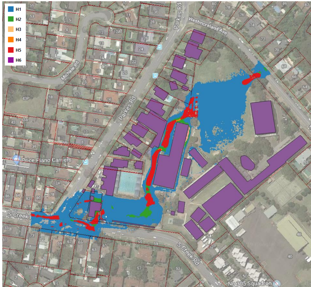
Figure 19 - Pre-development, 1% AEP (blocked), Flood Hazard
