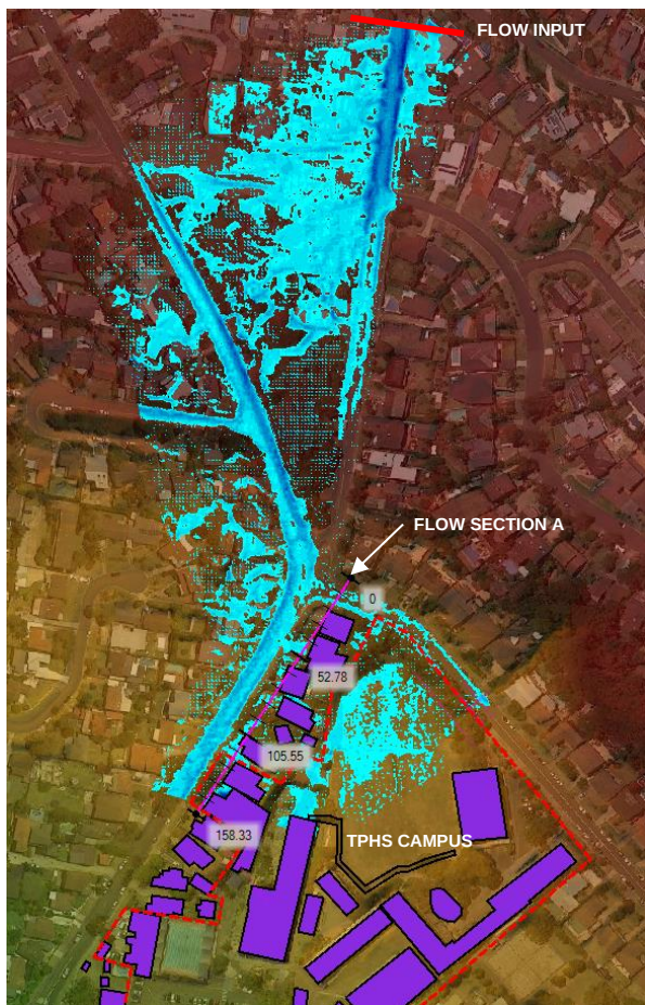
Figure 5 - Catchment A, PMF, Depth, contributing flows
