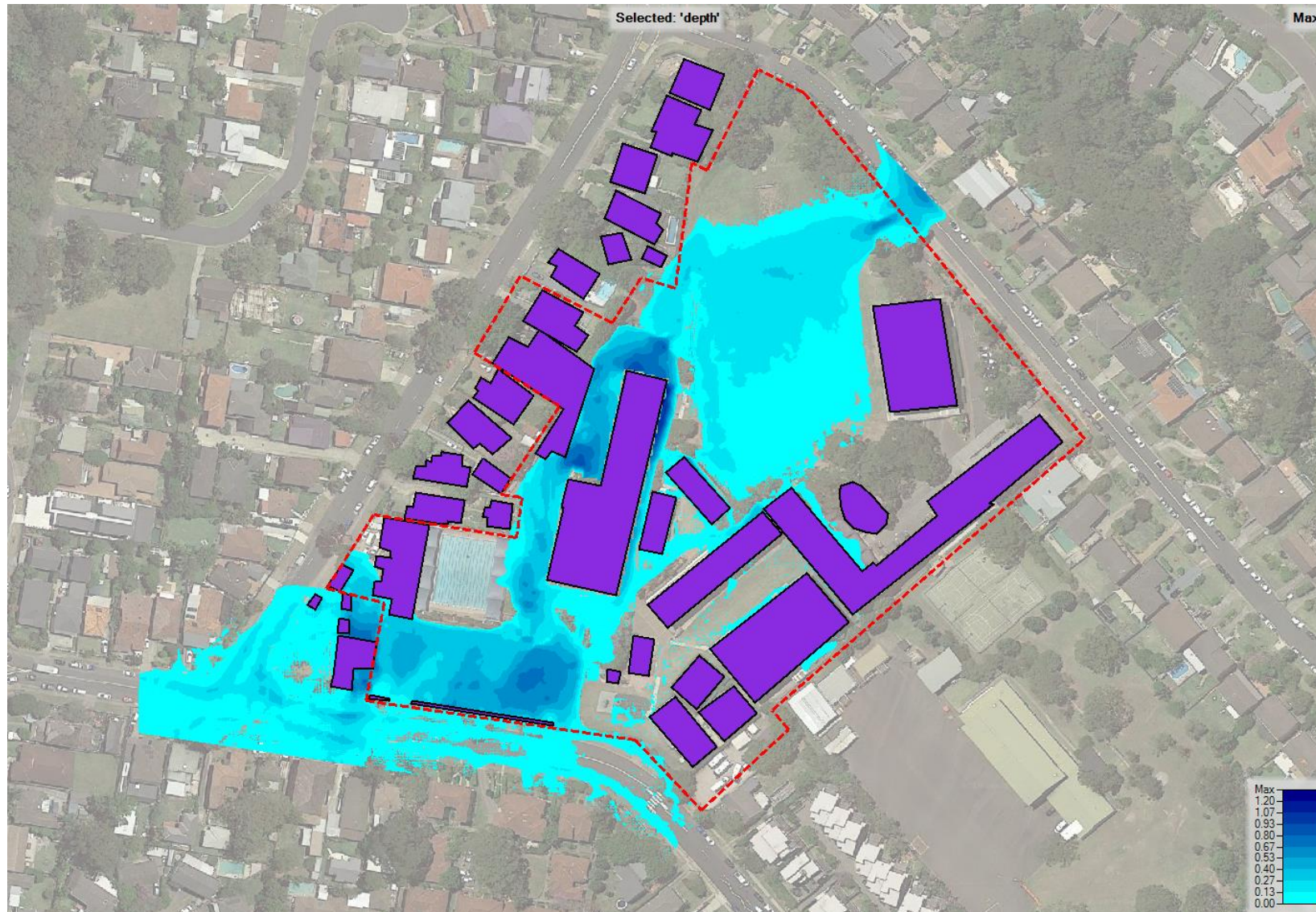
Figure 20 - Pre-development, PMF, Depth (m)
