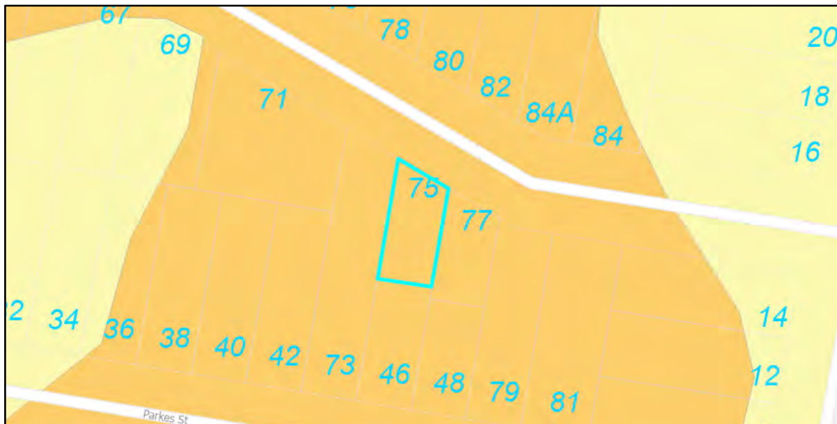
Figure 1. Warringah Landslip Risk Map: 75 Innes Road, Manly Vale NSW (© NBC Maps)
