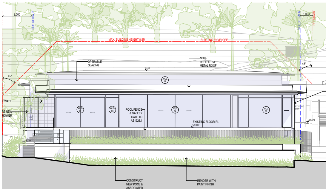
01 EAST ELEVATION
