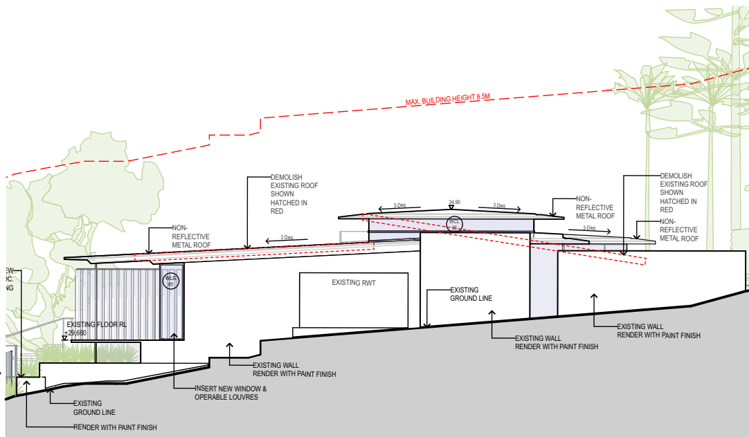
02 NORTH ELEVATION
