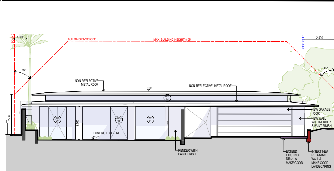
04 WEST ELEVATION
