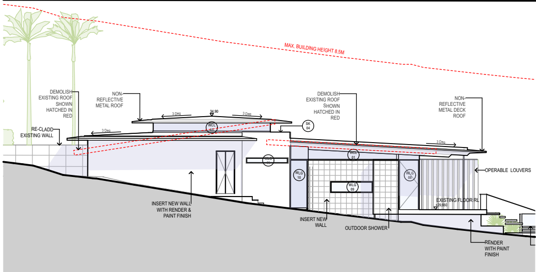
03 SOUTH ELEVATION
