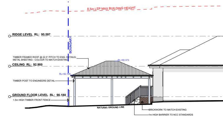
NORTH ELEVATION 1:200
