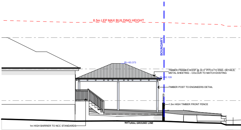
WEST ELEVATION 1:200
