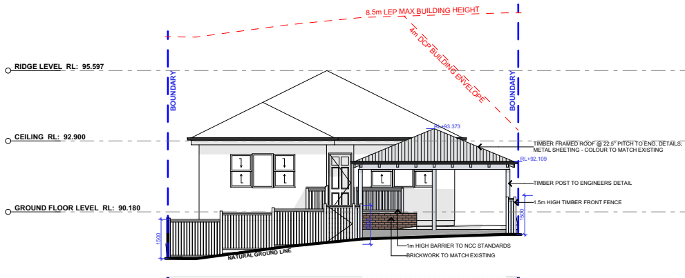
EAST ELEVATION 1:200
