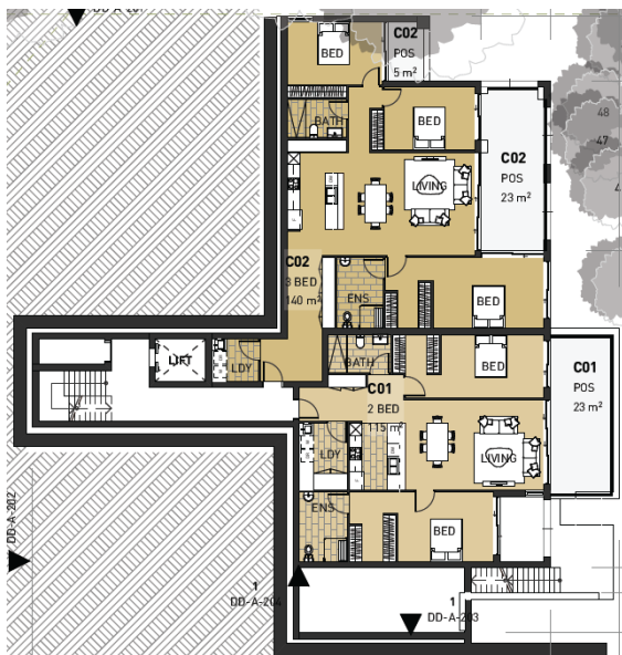
Building C Level 0
