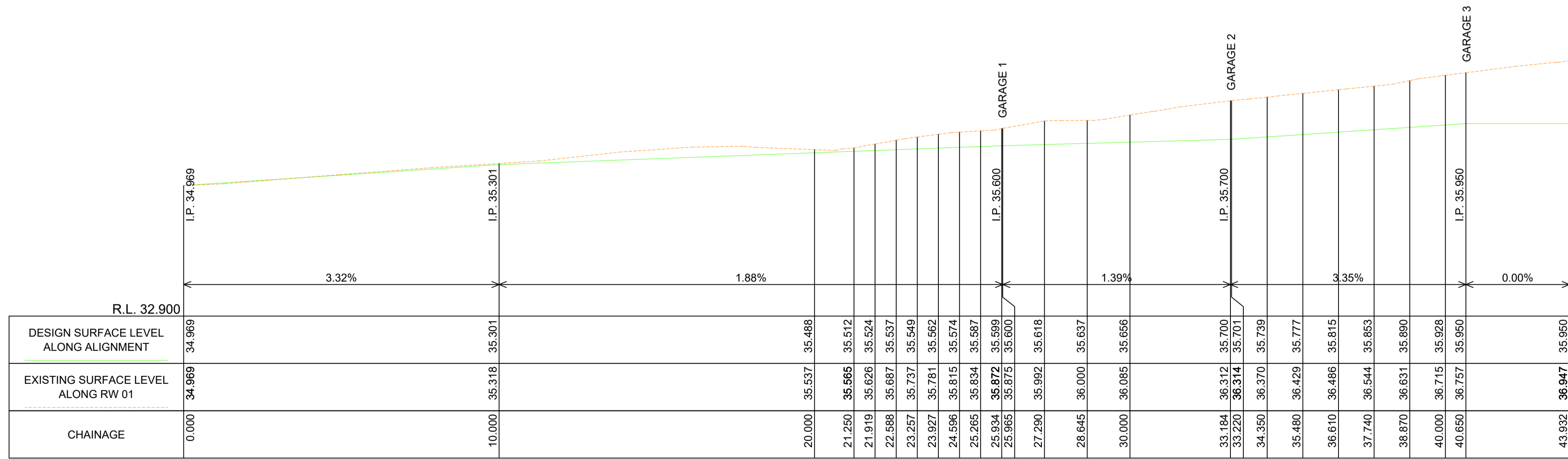
LONGITUDINAL SECTION ALONG LS01-DRIVEWAY SCALE H:1in100 V:1in50
