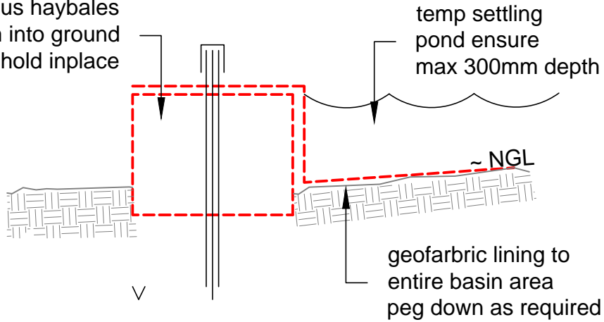
HAY BALE / SETTLING POND DETAIL
