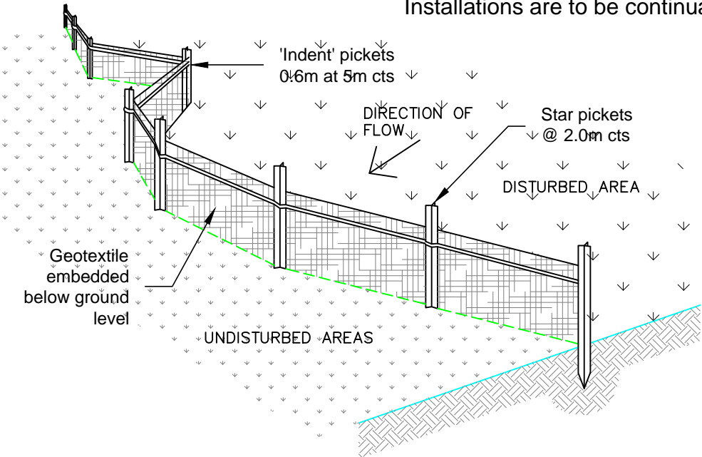
SEDIMENT FENCE
