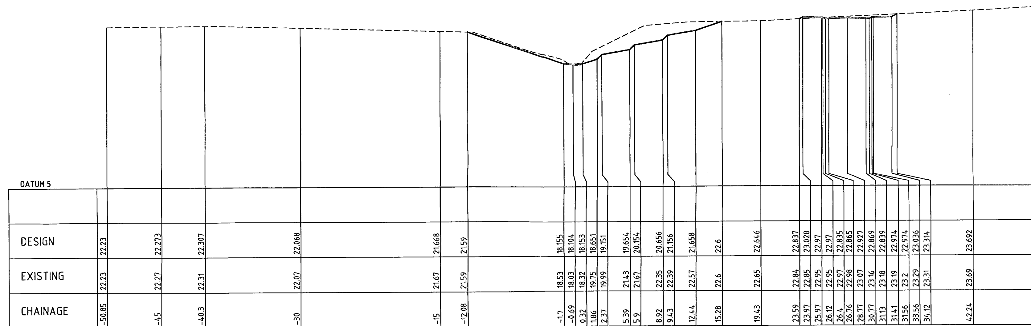
SECTION C9 SCALE 1:250
