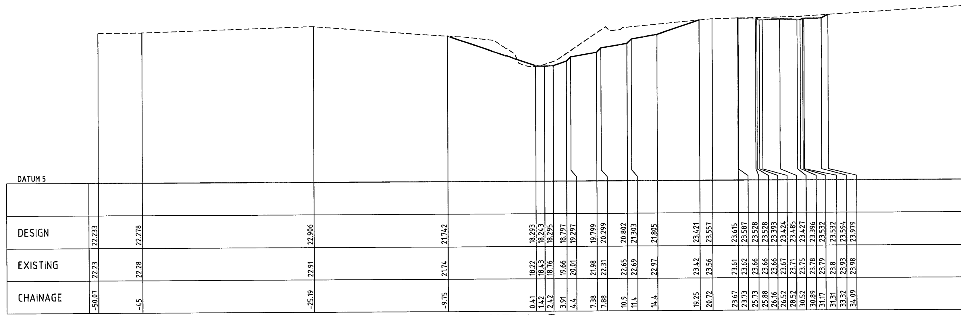
SECTION C9 SCALE 1:250
