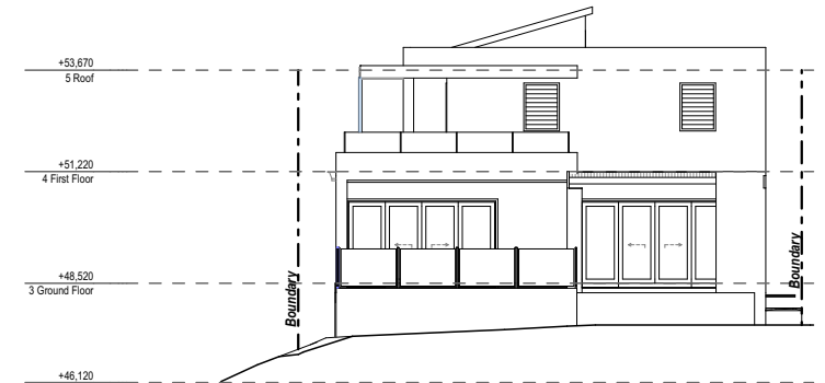
East Elevation
