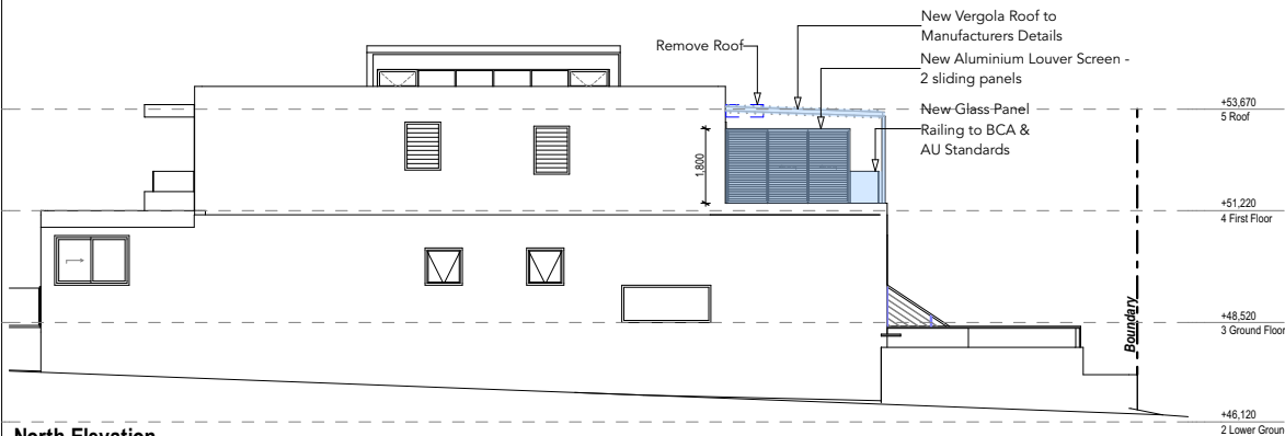
North Elevation
