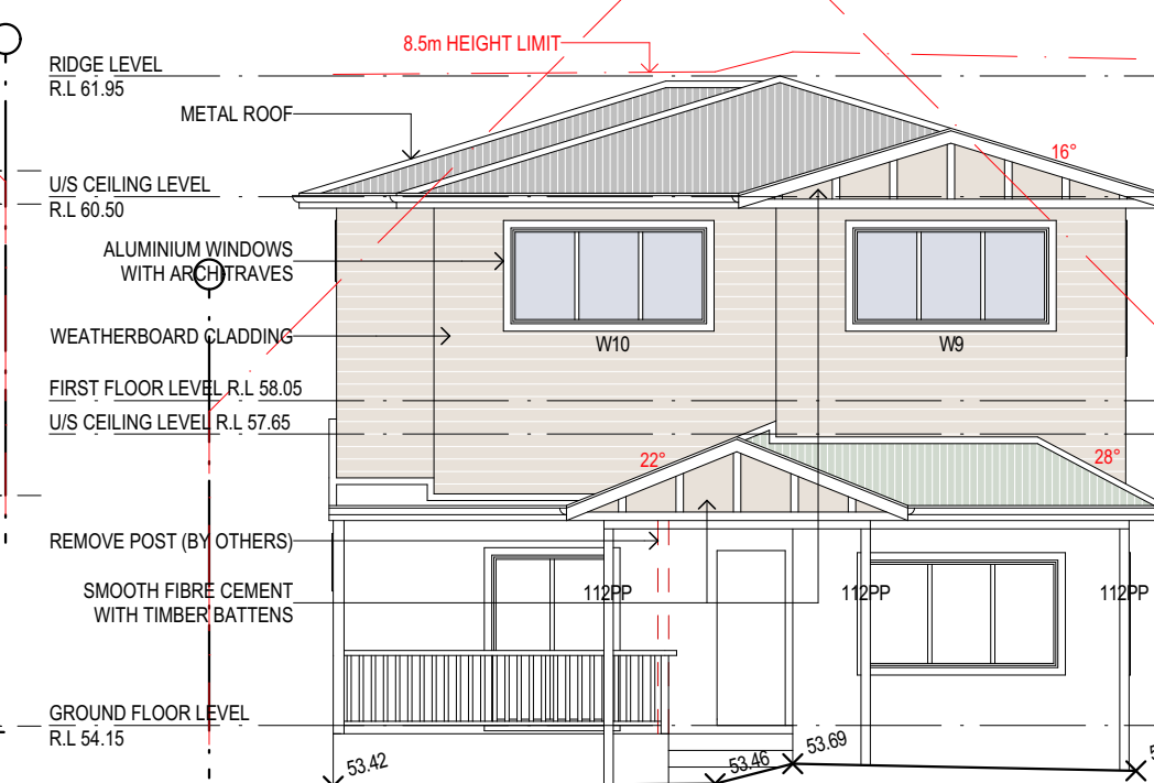
WEST ELEVATION
