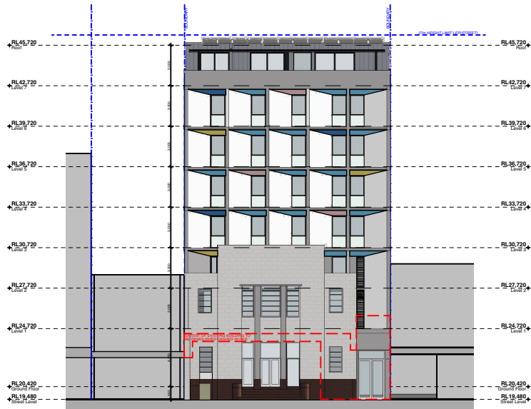
Notification_SE Elevation 1:400
