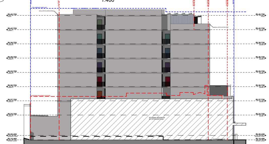
Notification_E Elevation 1:400
