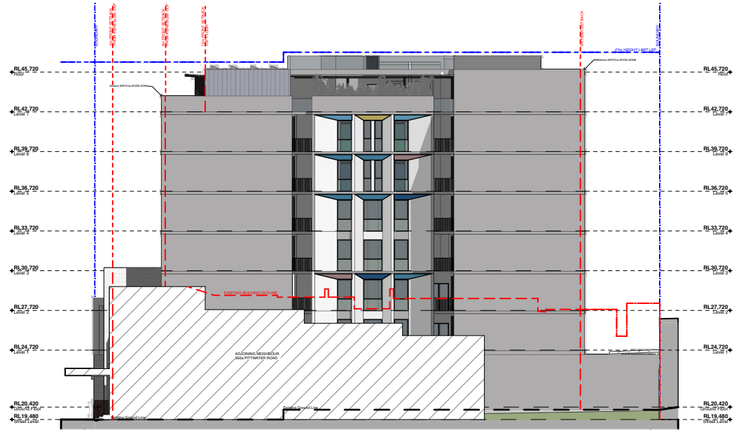
Notification_E Elevation 1:400
