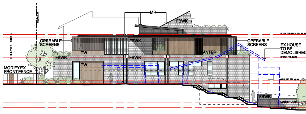
West Elevation
