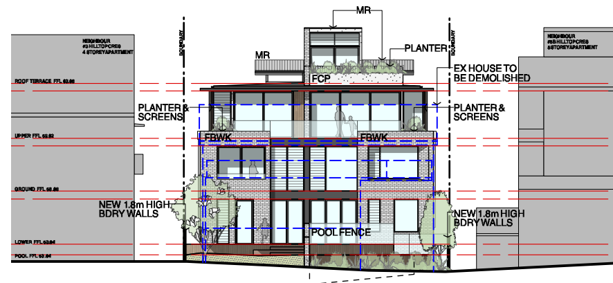
South Elevation
